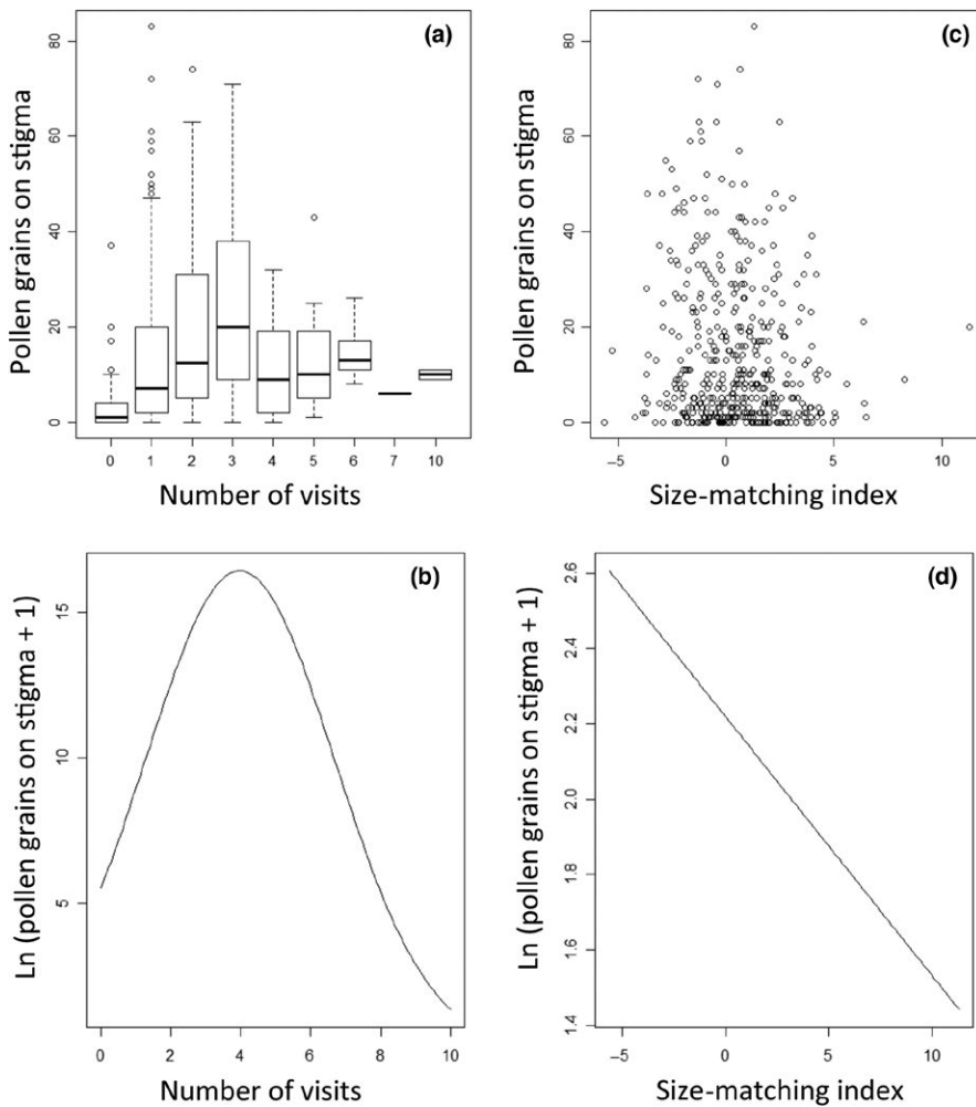
FIGURE 4 Pollen grains deposited on the stigma of Solanum rostratum as a function of (a) the number of visits conducted by Bombus terrestris , and (c) the size-matching index, which measures the fit between the pollinator and the visited flower (positive values indicate that the distance between the floral sexual organs is larger than the width of the abdomen of the floral visitor). Lower panels show the fitted lines of the best-fitting regression models of natural log-transformed pollen grains on stigma [ \ln(\text{pollen grains} + 1) ], as a function of (b) number of visits (quadratic model), and (d) the size-matching index (linear model)
