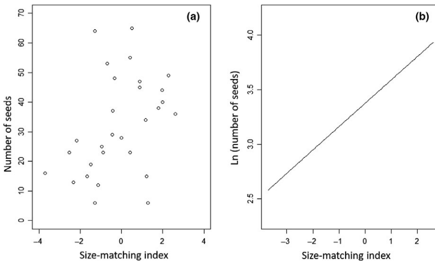
FIGURE 5 (a) Scatterplot showing the number of seeds produced by individuals fruits of the experimental plants against the size-matching index between flowers of Solanum rostratum and Bombus terrestris . (b) Fitted line of the regression model on natural-log transformed number of seeds [ \ln(\text{number of seed}) ]
