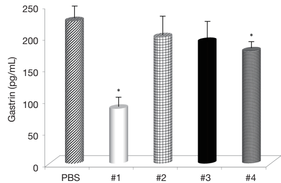
Figure 4 Effects of curcumin on serum levels of gastrin. Results represent mean from three experiments \pm SD. *, represents significant differences between the control and curcumin-treated mice at P \leq 0.05 level.
