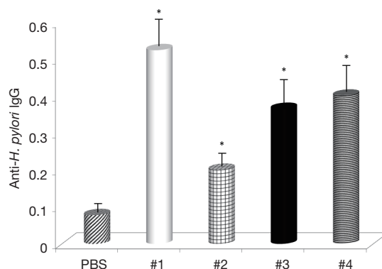
Figure 7 Effects of curcumin on anti- H. pylori IgG formation. Results represent mean from three experiments ± SD. *, represents significant differences between the control and curcumin-treated mice at P<0.05 level.
