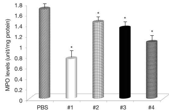
Figure 6 Effects of curcumin on MPO activity in gastric mucosal tissue. Results represent mean from three experiments \pm SD. *, represents significant differences between the control and curcumin-treated mice at P \leq 0.05 level. MPO, myeloperoxidase.
