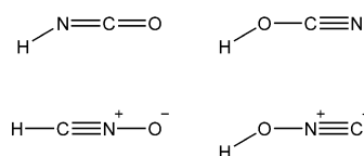
Scheme 1. Known isomers in the HNCO system.
