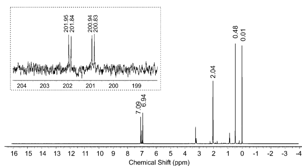
Figure 2. ^1\text{H} NMR spectrum of HPCO ( [\text{D}_8] toluene, 223 K). Inset: ^{13}\text{C} NMR spectrum.
