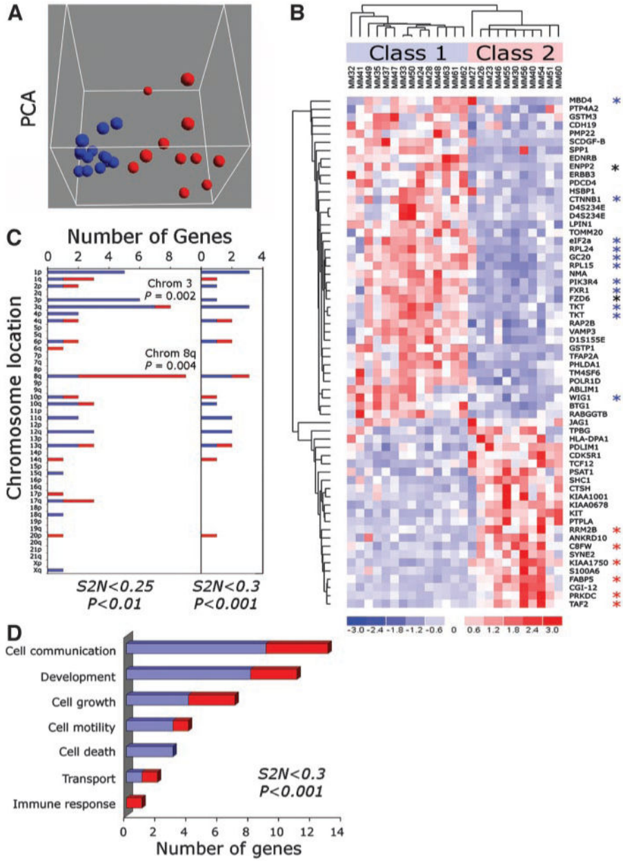
Fig. 1. Gene expression profile analysis of primary uveal melanomas reveals two distinct tumor classes. A , principal component analysis (PCA) demonstrating a tight cluster of 14 tumors ( blue spheres ; class 1) and a distinct cluster of 11 tumors ( red spheres ; class 2). B , hierarchical clustering heat map of 62 discriminating genes with an absolute signal-to-noise (S2N) score > 0.25 and P < 0.01 . Class 1 (low-grade) and class 2 (high-grade) tumors are indicated. Blue asterisks indicate chromosome 3 genes that are down-regulated in class 2, red asterisks indicate chromosome 8q genes that are up-regulated in class 2, and black asterisks indicate chromosome 8q genes that are down-regulated in class 2. C , chromosomal distribution of the top 62 ( left panel ) and top 26 ( right panel ) discriminating genes with
