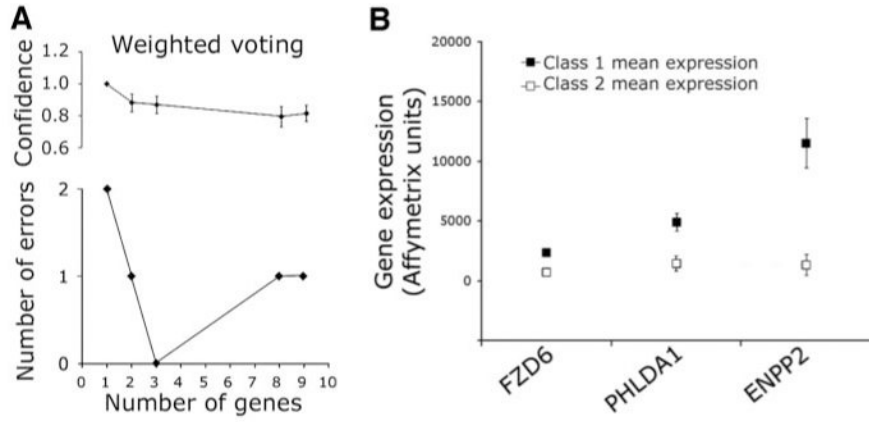
Fig. 2. Supervised training models identify a three-gene signature that accurately predicts tumor class. A , correct assignments and confidence scores (with SE) using a weighted voting algorithm. The performance of the model is indicated as a function of the number of genes included in the model. As few as three genes assign all tumors to the correct class with no improvement in performance by including additional genes. B , comparison of mean Affymetrix gene expression values in class 1 versus class 2 tumors for the 3 signature genes ( error bars indicate SE).
