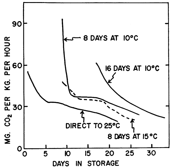
FIG. 3. Effect on respiratory rate of transferring cucumber fruits from a lower temperature to 25^\circ\text{C} . Left —The effect of prior holding at 5^\circ\text{C} . Right —The effect of prior holding at 10 and at 15^\circ\text{C} .
