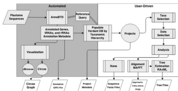
Fig. 1. Verdant workflow. Workflow diagram depicting the automated (grey box) and user-driven (white box) steps and options available in Verdant. Parallelograms at the bottom of the diagram represent downloadable files available
