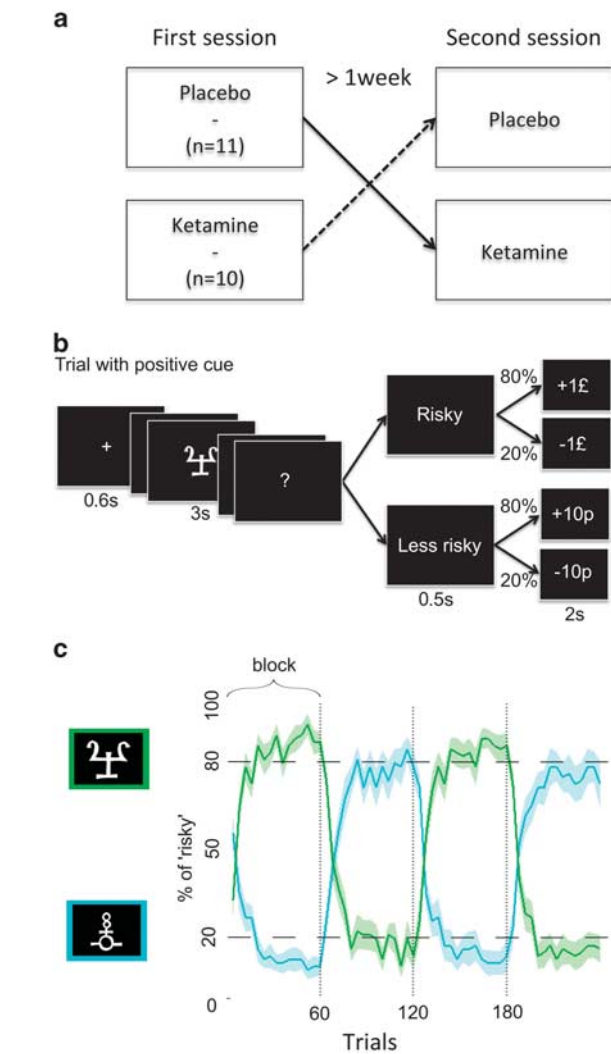
Figure 1. Experimental design. (a) A double-blind, placebo-controlled, randomized, within-subject design was used. The order of drug and placebo visits was counterbalanced across subjects and spaced by at least 1 week. (b) A typical trial and possible outcomes for a positive cue. Probabilistic contingencies (80 and 20%) would be swapped for a negative cue. (c) Percentage of risky responses as a function of trial number (both placebo and ketamine sessions were pooled). The green (respectively, blue) curve represents the choices following the cue that was positive (respectively, negative) in the first block. Bold lines represent means; color-delimited areas represent inter-subject s.e.m. (corrected for the variance across subject: the grand mean of each subject was removed from its data before computing sem). Vertical dashed lines indicate reversals.
