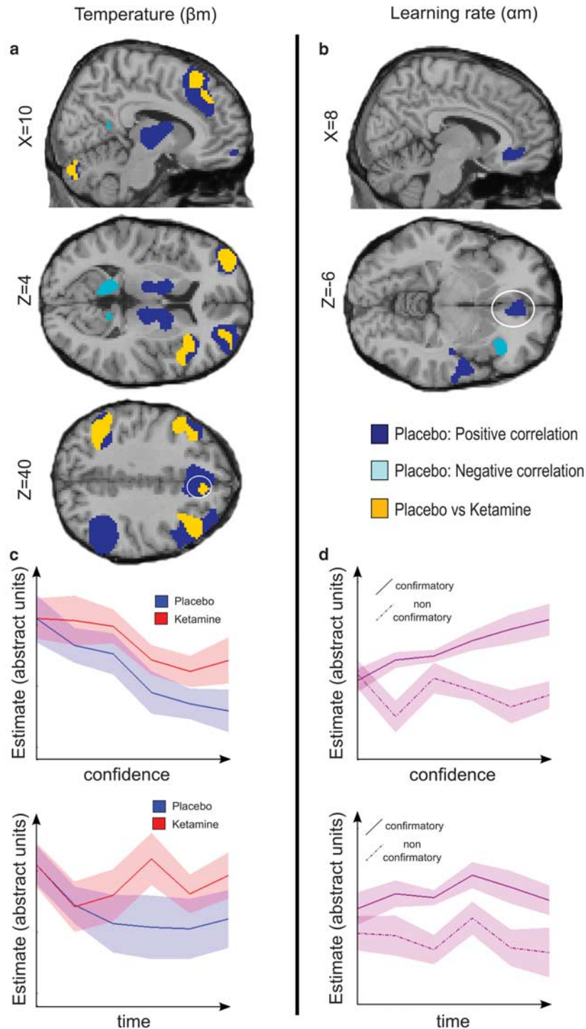
Figure 5. Model-based analysis of ketamine-induced changes in brain activity (a) Brain regions reflecting confidence-modulated choice temperature ( \beta_m ). (b) Brain regions reflecting confidence-modulated learning rate ( \alpha_m ). Colored clusters show significant correlation in the placebo session (positive in dark blue, negative in light blue) and significant difference between placebo and ketamine sessions (in orange). All clusters survived a statistical threshold of P < 0.05 after family wise error correction for multiple comparisons. Coordinates of anatomical slices are given in Montreal Neurological Institute space. (c) Hemodynamic response to cue onset in the dmPFC as a function of confidence bins or as a function of time (trial number, pooled across blocks) (for illustrative purpose). (d) Hemodynamic response to outcome onset in the ventromedial prefrontal cortex as a function of confidence bins or as a function of time (trial number, pooled across blocks) (for illustrative purpose), shown separately for confirmatory and contradictory outcomes. Placebo data are in blue, ketamine data are in red, pooled data are in violet. Bold lines represent means; color-delimited areas represent inter-subject s.e.m (corrected for the variance across subject: the grand mean of each subject was removed from its data before computing s.e.m.).
