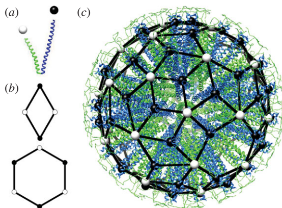
Figure 1. SAPN architecture and nanoparticle graphs. (a) The SAPN building blocks consist of two fused polypeptide helices, that cluster in groups of three (black sphere) and five (white sphere) in the nanoparticle shell. (b) Nanoparticle graphs correspond to spherical tessellations in terms of rhombs and hexagons, with vertices labelled alternately by black and white spheres. (c) A SAPN formed from 180 PBBs, together with its nanoparticle graph (adapted from a figure by N. Wahome and P. Burkhard). The nanoparticle model was built using a variety of adapted tools from the CCP4 program suite ( www.ccp4.ac.uk/ ), the modelling software O ( xray.bmc.uu.se/ ) and data from the RCSB database ( www.rcsb.org/ ). The nanoparticle graph has been obtained by modifying a fullerene graph of the library of the FULLERENE PROGRAM [18].
