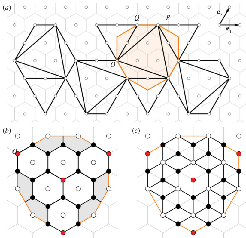
Figure 4. (a) The Fowler–Cremona–Steer construction for fullerenes with tetrahedral symmetry. Here O = (0, 0) , P = (1, 2) , Q = (0, 2) with respect to the triangular lattice basis, so that (i, j) = (1, 2) and (h, k) = (0, 2) . The domain used here for the construction of the nanoparticles (corresponding in area to three times the fundamental domain) is shown highlighted; (b) a close up at this domain for the case of fullerene C_{68} , with areas corresponding to portions of six of the 12 pentagons of the fullerene shown in grey; and (c) close-up of the domain in the corresponding nanoparticle graph ( N = 180 ), with trimers deleted according to the vertex colouring rule shown in red.
