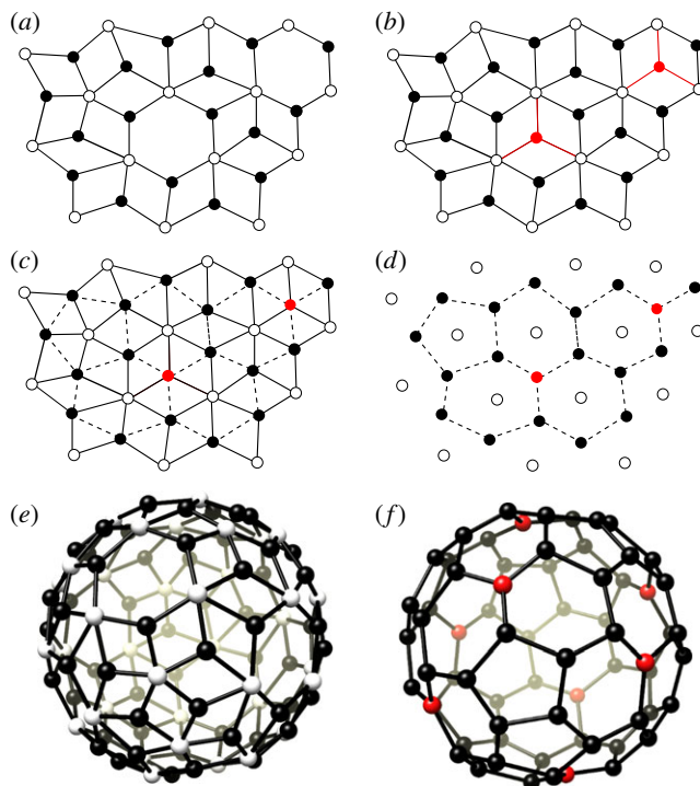
Figure 2. The vertex addition rule for the construction of the fullerene equivalent of a nanoparticle graph. (a) A portion of a nanoparticle graph; (b) the vertex addition rule adds additional three-coordinated vertices (red) at the centres of the hexagonal faces with connections to the five-coordinated vertices (white) of the nanoparticle graph; (c) pairs of trimers belonging to the same rhomb are connected by a dashed line; (d) removal of all edges of the nanoparticle graph in (a) results in a fullerene graph; (e) the nanoparticle graph for a particle with N = 180 PBBs; and (f) the fullerene graph C_{68}(T_d) obtained via the vertex addition rule, with red points representing the trimers added to the nanoparticle graph in the procedure.
