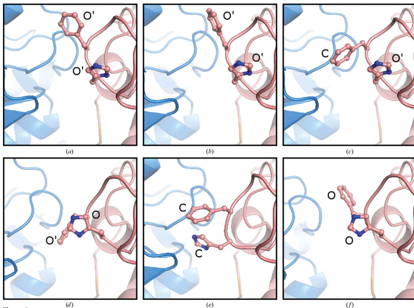
Figure 3 Comparison of the side-chain conformations of the MG residues in (a) the Ado-complexed subunit of the Ado/Cord complex, (b) subunit A of the Ado complex, (c) subunit B of the Ado complex, (d) the Cord-complexed subunit of the Ado/Cord complex, (e) subunit A of the Ade complex and (f) the open subunit (D) of PDB entry 4lvc. The side chains of the molecular-gate residues His342 and Phe343 are shown in ball-and-stick representation and annotated as C (closed state), O (open state) or O' (variant open state; see text).
