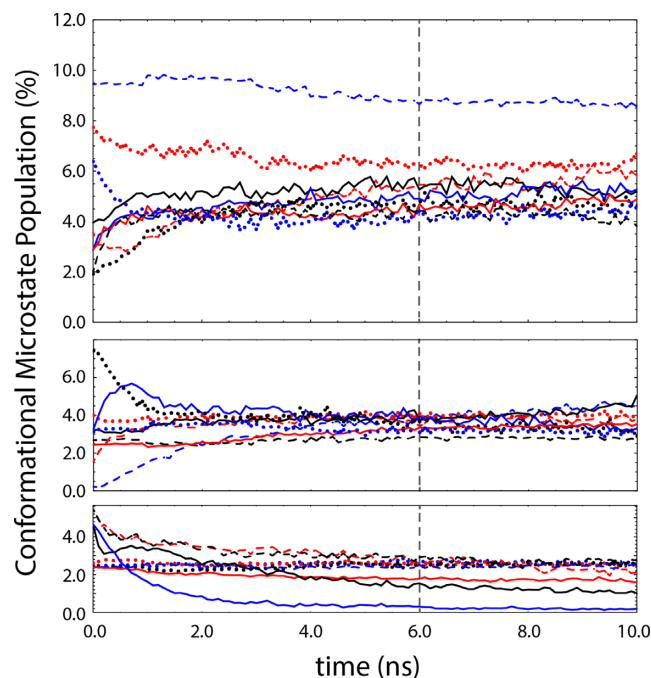
Figure 3. Populations of the 27 conformational microstates identified by K -means clustering versus time (split into three panels for visual clarity). Approximate conformational equilibrium is established at 6.0 ns (dashed line).
