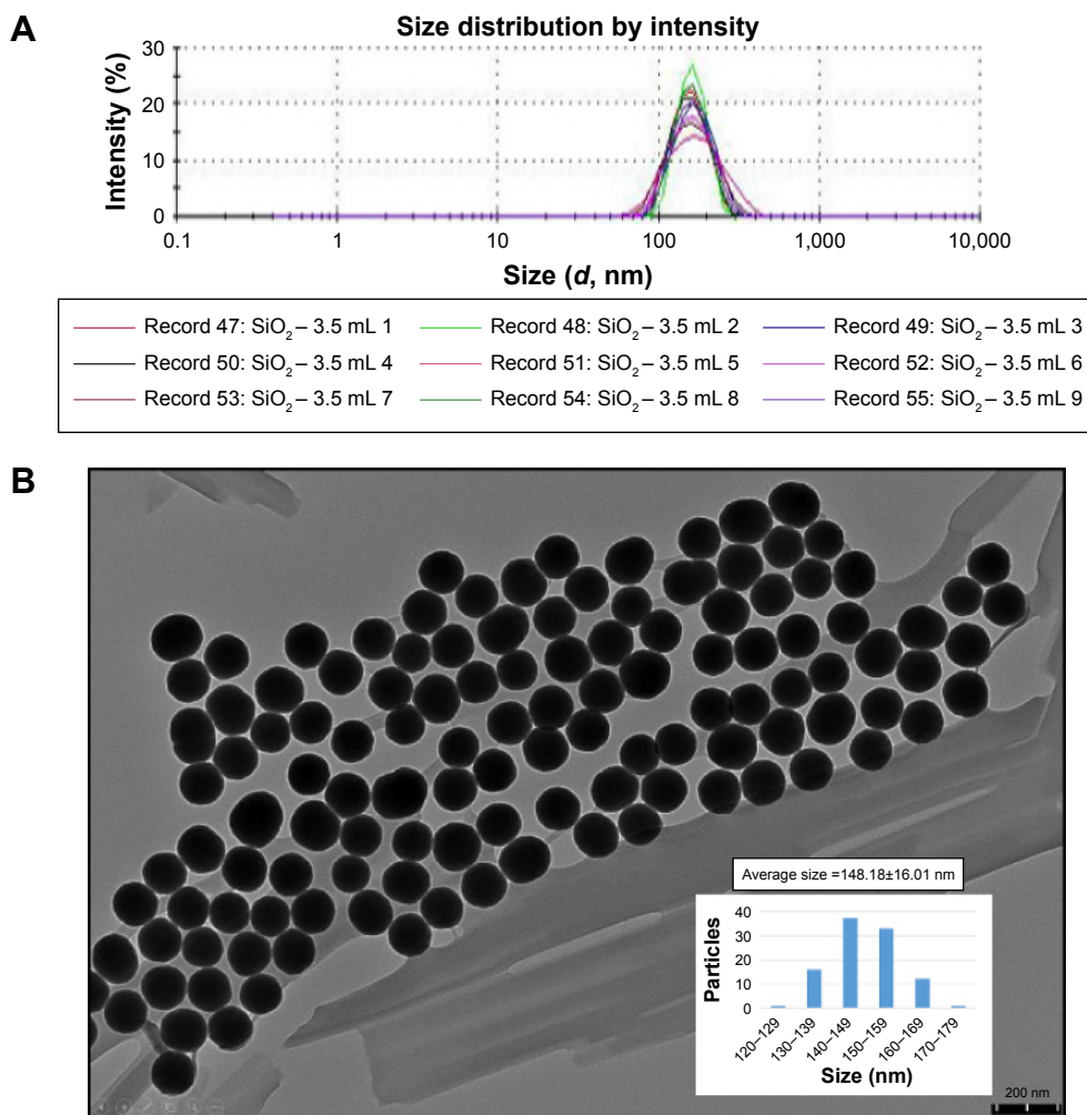
Figure 1 Characterization of SiNPs. Notes: (A) DLS size distribution with an average diameter of ~153.8 nm. (B) TEM images showed the SiNPs in near-spherical shape with well dispersibility with an average diameter of ~148.18 nm. Abbreviations: DLS, dynamic light scattering; SiNPs, silica nanoparticles.
