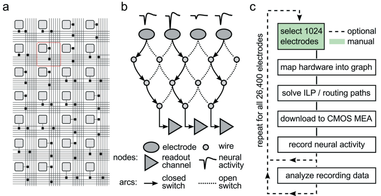
Fig. 2. Reconfigurable Electrode Array.
