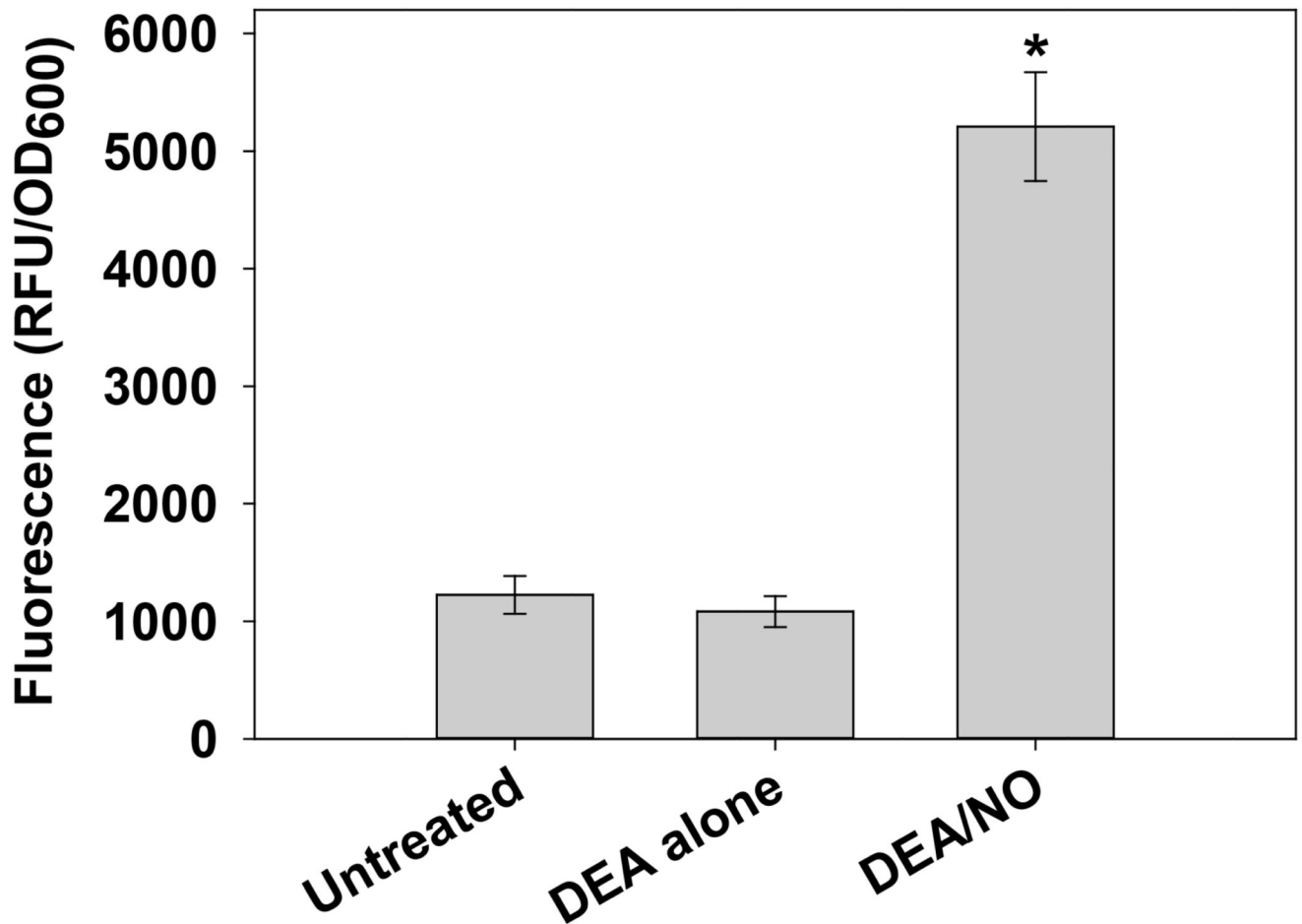
Figure 2. Detection of intracellular NO/RNS in S. aureus with DAF-FM diacetate
