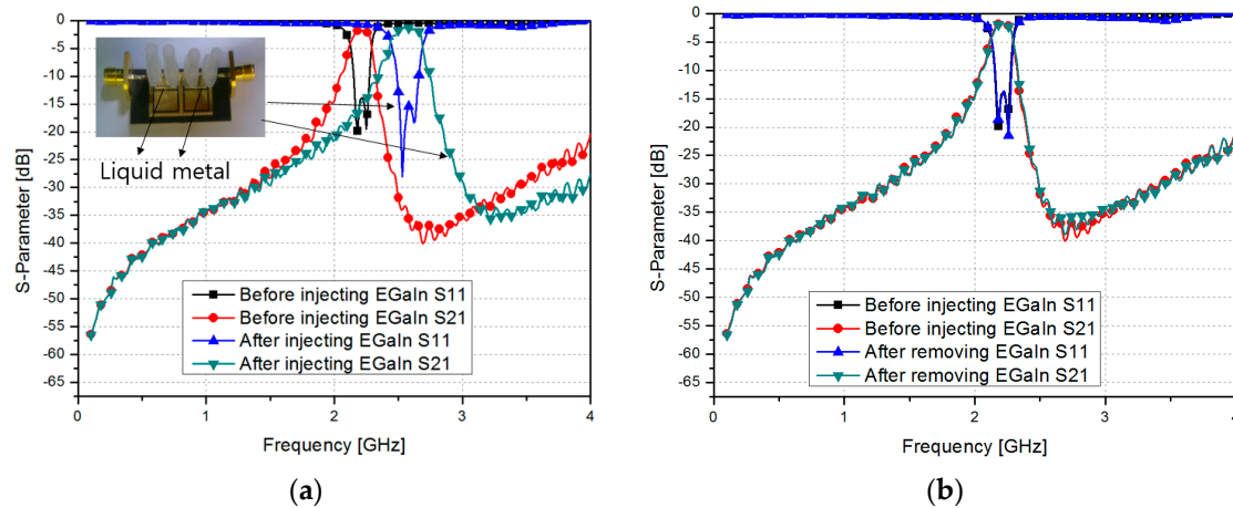
Figure 10. Measured S-parameter of the fabricated CSRR-loaded QMSIW (a) before and after injecting the microfluidic channels with EGaIn; and (b) before injecting EGaIn and after the removal of EGaIn.
