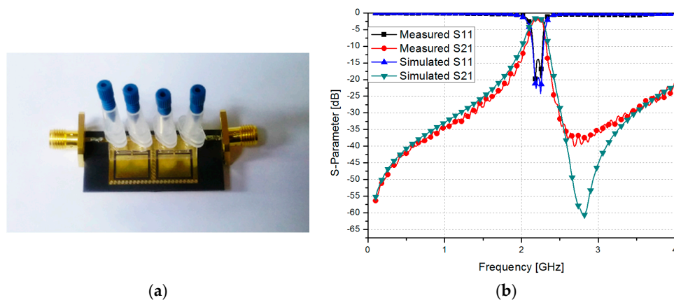
Figure 9. (a) Fabricated CSRR-loaded QMSIW filter prototype and (b) simulated and measured S-parameter of the proposed CSRR-loaded QMSIW filter.
