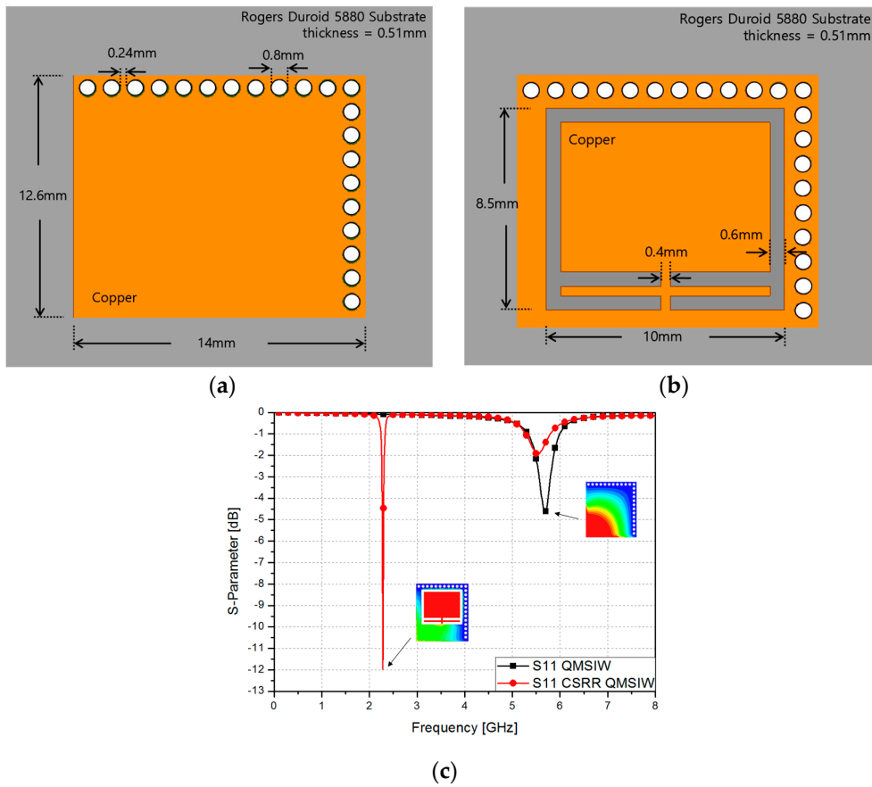
Figure 2. Geometry of (a) QMSIW and (b) CSRR-loaded QMSIW; (c) simulated S-parameters of CSRR-loaded QMSIW and QMSIW with the E-field distribution layout.
