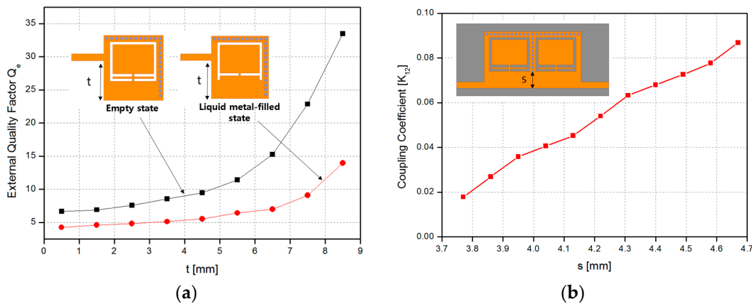
Figure 3. (a) External quality factor variation with distance t for the CSRR-loaded QMSIW resonator. (b) The coupling coefficient of coupled cavities with distance s .
