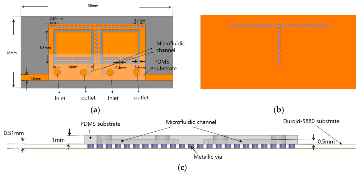
Figure 4. (a) Top view of the CSRR-loaded QMSIW filter with a PDMS substrate; (b) bottom view of the proposed filter; and (c) side view of the proposed filter.
