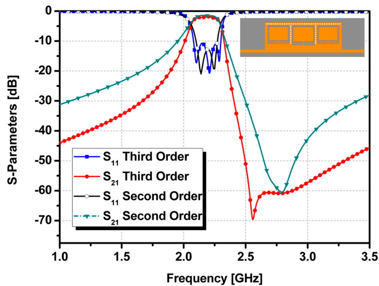
Figure 6. Designs of second-order and third-order CSRR-loaded QMSIW band-pass filters and their simulated S-parameter results.
