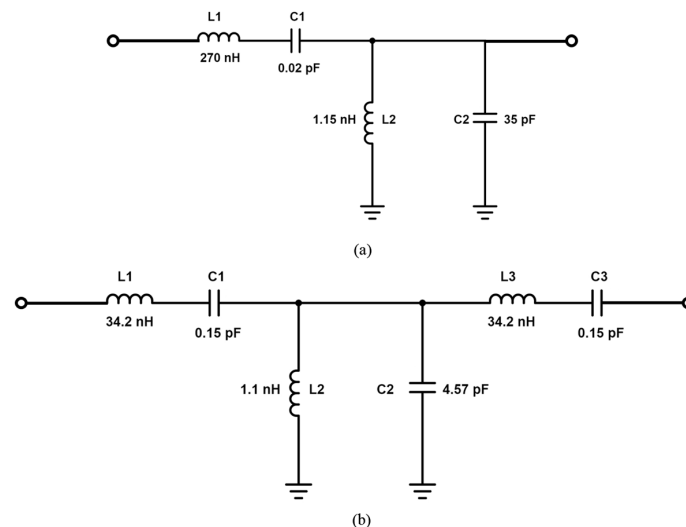
Figure 7. Equivalent circuits of (a) proposed second-order band-pass filter design and (b) third-order bandpass filter design shown in Figure 6.
