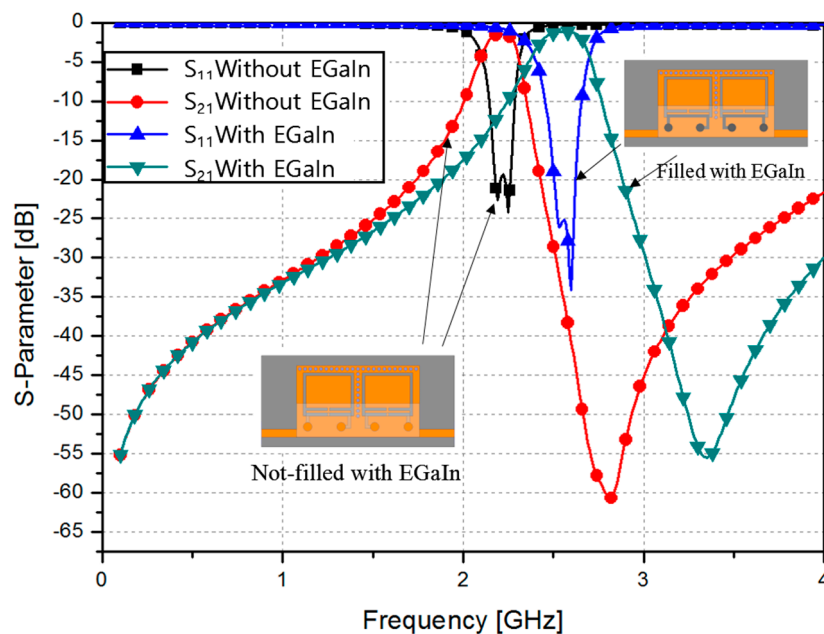
Figure 5. Simulated S-parameter of the CSRR-loaded QMSIW before and after injecting EGaIn.
