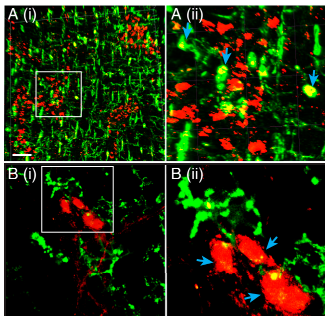
Fig. 3. Muscularis macrophages phagocytose myenteric neurons in healthy guts. (A, i ) Two-photon microscopy of myenteric plexus from the colon of a ChAT-cre:tdTomato mouse shows tdTomato-expressing (red) cholinergic neurons along with MHC class II-labeled muscularis macrophages (green) shows an abundance of macrophages associated with the myenteric plexus. Inset (i) is magnified and shows (ii) the engulfment of tdTomato-expressing neuronal soma (red) in MHC II labeled macrophages (green; cyan arrows). (Scale bar, 50 \mu\text{m} .) (B, i ) A 2D projection image of a z-stack of confocal microscopy images of neurons within the small intestinal myenteric ganglia shows the colocalization of ChAT-cre:tdTomato (red) signal along with that of CD11b-stained (green) muscularis macrophages. Inset (i) is magnified and shows (ii) the engulfment of tdTomato-expressing neuronal soma (red) by CD11b-stained macrophages (green; cyan arrows), suggesting phagocytosis of myenteric neurons by macrophages. (Scale bar, 10 \mu\text{m} .)
