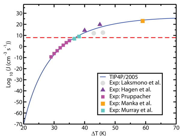
Figure 16. Nucleation rate J as determined for the TIP4P/2005 model (blue solid line) compared to experiments (filled squares) of Pruppacher, 255 Murray et al., 246 and Manka et al. 256 Experimental results from Laksmo et al. 248 (filled circles) and Hagen et al. 247 (filled triangles) were also included. The horizontal line corresponds to \log_{10} J (\text{cm}^{-3} \text{ s}^{-1}) = 8 , which is the approximate value of J at the homogeneous nucleation temperature in experiments (i.e., about 38 K below the melting point). Figure adapted with permission from ref 235. Copyright 2014 American Institute of Physics.
