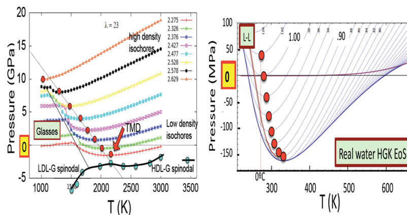
Figure 30. (Left) Behavior of the isochores and the TMD with isochores density in the tuned S–W model with \lambda parameter = 23. The TMD does not reverse as it does for the silicon potential \lambda = 21 . Flattened segments at lower temperatures correspond to broken ergodicity states (glasses on the simulation time scale). (Right) Isochores and density maxima behavior of the HGK equation of state for water.
