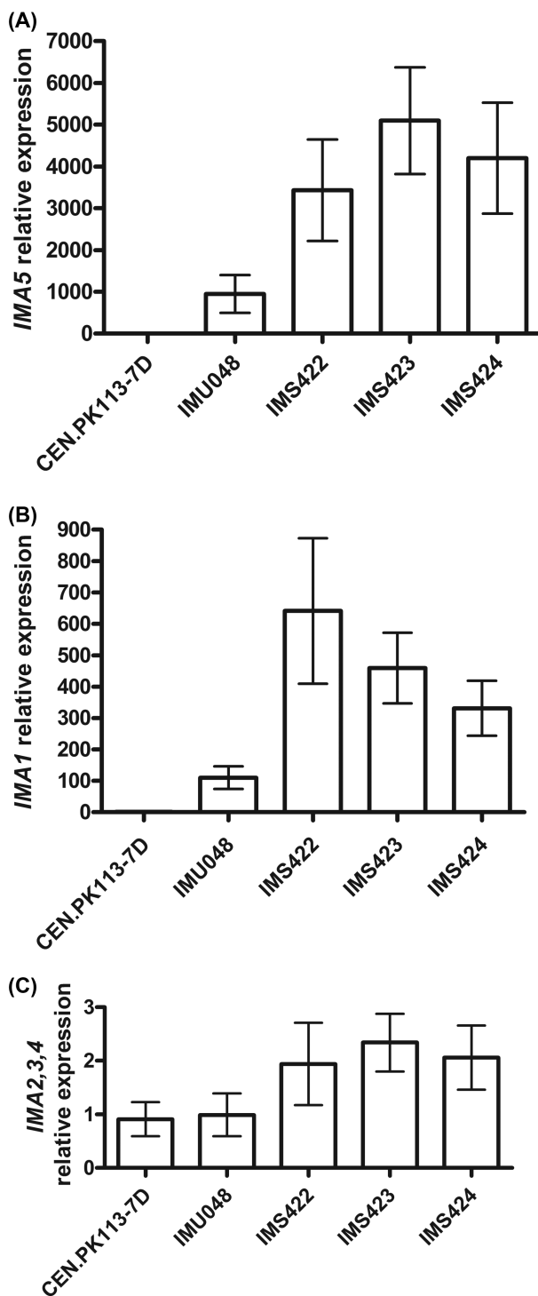
Figure 3. Relative expression of IMA1-5 in S. cerevisiae strains evolved for faster growth on SM with sucrose as the sole carbon source. Relative expression of IMA5 (A); IMA1 (B); and IMA2, IMA3 and IMA4 (C). Expression of IMA2, IMA3 and IMA4 was assayed by a single primer pair since these genes are highly similar in nucleotide sequence. CEN.PK113-7D: reference strain ( IMAx MALxx MPHx SUC2 ); IMU048: unevolved parental strain (genotype: malΔ mphΔ suc2Δ MAL11 ); and three independently evolved strains (IMS422, IMA423 and IMS424). CEN.PK113-7D was used as calibrator sample (expression set to 1). Averages and standard errors were obtained from independent duplicate biological experiments and three technical replicates. Cells were harvested at mid-exponential phase ( OD_{600nm} = 3 ) from shake-flask cultures on SM with sucrose as sole carbon source.
