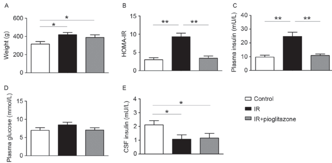
Figure 1. Pioglitazone treatment improves insulin sensitivity in HD-induced IR rats. Rats were assessed following 16 weeks (12 weeks to establish the IR model plus 4 weeks treatment/HD-diet) on a normal or HD diet for different indices of HD-induced IR, including: (A) Body weight, (B) HOMA-IR, (C) plasma insulin, (D) plasma glucose and (E) CSF insulin. Data are presented as the mean \pm standard deviation. Control group, n=10; IR model rat groups, n=8/group. *P<0.05 and **P<0.01. CSF, cerebrospinal fluid; HD, high glucose, high fat and high protein diet; HOMA-IR, homeostasis model assessment-insulin resistance; IR, insulin resistance.
