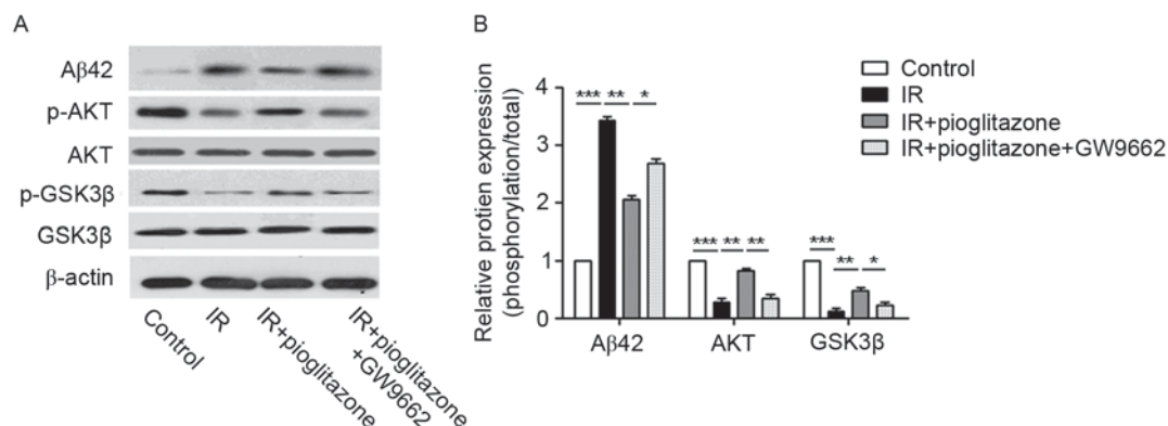
Figure 5. GW9662 reverses inhibiting effect of Pioglitazone on A \beta 42 deposition in IR model rats via AKT/GSK3 \beta signaling pathway. (A) Western blot analysis of the protein expression of A \beta 42 and components of the AKT/GSK3 \beta signaling pathway in the different experimental rat groups. (B) Densitometric analysis of the bands in (A), all normalized to \beta -actin. Control group, n=10; IR model rat groups, n=8/group. Data are presented as the mean \pm standard deviation. *P<0.05, **P<0.01 and ***P<0.001. A \beta 42, amyloid \beta , isoform 42; p-, phosphorylated; AKT, protein kinase B; GSK3 \beta , glycogen synthase kinase 3 \beta ; GW9662, peroxisome proliferator-activated receptor \gamma inhibitor; IR, insulin resistance.
