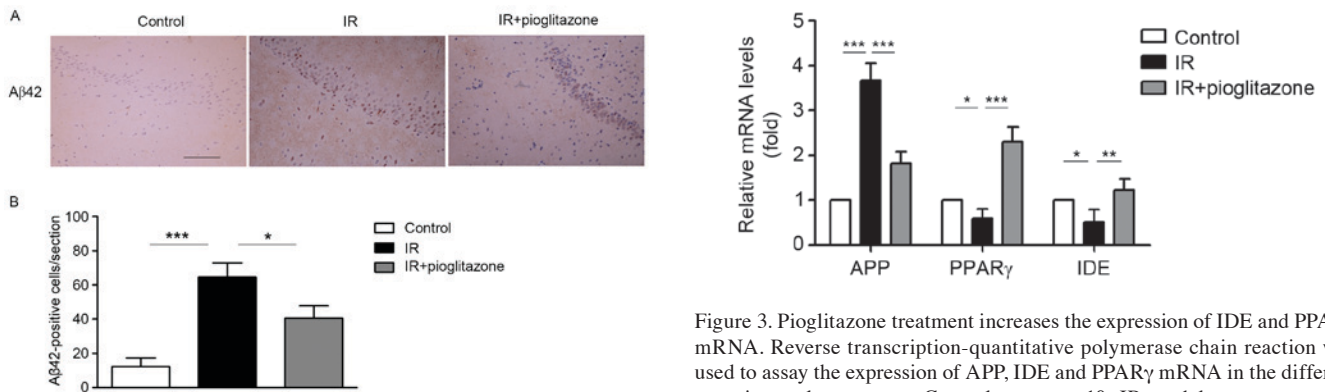
Figure 2. Pioglitazone treatment alleviates A \beta 42 accumulation in the hippocampus of IR model rats. (A) Immunohistochemical analysis of A \beta 42 in the hippocampus of the different rat groups. Scale bar, 100 \mu m. (B) A \beta 42-positive cells were increased in IR model rats compared with control, but decreased following pioglitazone treatment. Data are presented as the mean \pm standard deviation. Control group, n=10; IR model rat groups, n=8/group. *P<0.05 and ***P<0.001. A \beta 42, amyloid \beta , isoform 42; IR, insulin resistance.
