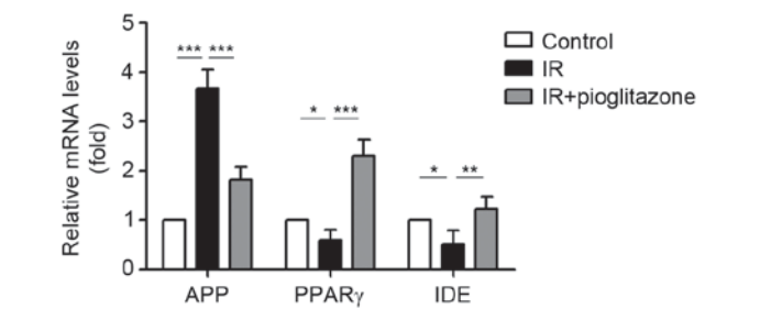
Figure 3. Pioglitazone treatment increases the expression of IDE and PPAR \gamma mRNA. Reverse transcription-quantitative polymerase chain reaction was used to assay the expression of APP, IDE and PPAR \gamma mRNA in the different experimental rat groups. Control group, n=10; IR model rat groups, n=8/group. Data are presented as the mean \pm standard deviation. *P<0.05, **P<0.01 and ***P<0.001. APP, amyloid precursor protein; IDE, insulin-degrading enzyme; IR, insulin resistance; PPAR \gamma , peroxisome proliferator-activated receptor \gamma .
