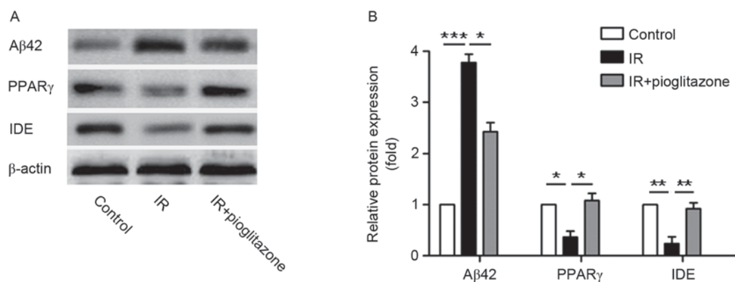
Figure 4. IDE and PPAR \gamma are involved in the inhibitory effect of pioglitazone on A \beta 42 accumulation. (A) Western blot analysis of the protein expression levels of A \beta 42, IDE and PPAR \gamma in the experimental rat groups. (B) Densitometric analysis of the bands in (A), normalized to \beta -actin. Control group, n=10; IR model rat groups, n=8/group. Data are presented as the mean \pm standard deviation. *P<0.05, **P<0.01 and ***P<0.001. IDE, insulin-degrading enzyme; PPAR \gamma , peroxisome proliferator-activated receptor \gamma .
