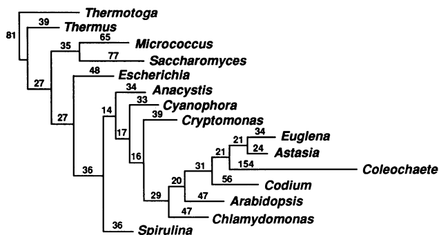
FIG. 3. The Coleochaete tufA is derived from a green algal chloroplast gene. The tree shown is the single shortest tree found by cladistic analysis of 15 eubacterial EF-Tu amino acid sequences. The tree has a total length of 1108 steps and a consistency index of 0.66, excluding autapomorphies. Thermotoga maritima , representing the earliest known branch of eubacteria (27), is used to root the tree. Horizontal branches are drawn to scale with lengths indicated numerically above the branches. tufA sequences in addition to those reported in Table 1 are Astasia longa (33), Micrococcus luteus (32), and Thermus thermophilus (34).
