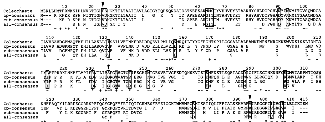
FIG. 2. Comparison of Coleochaete EF-Tu with EF-Tu consensus sequences. The Coleochaete deduced amino acid sequence is presented in its entirety together with consensus sites for cyanobacteria and chloroplasts (cp-consensus); eubacteria, cyanobacteria, and chloroplasts (eub-consensus); and eubacteria, eukaryotes, and archaeobacteria (all-consensus). The cp-consensus includes sites identical for 6 or more of 8 chloroplast and cyanobacterial sequences, the eub-consensus includes sites identical for 11 or more of 13 eubacterial and organellar sequences, and the all-consensus includes sites identical for 23 or more of 27 total sequences. Changes in the Coleochaete sequence relative to the consensus sequences are indicated below as very conservative (=), conservative (-), nonconservative (+), and very nonconservative (*) changes, as defined by Dayhoff et al. (21). Amino acid positions at which Coleochaete differs from all consensus sequences are enclosed in boxes. Sites specifically discussed in the text are denoted with arrowheads.
