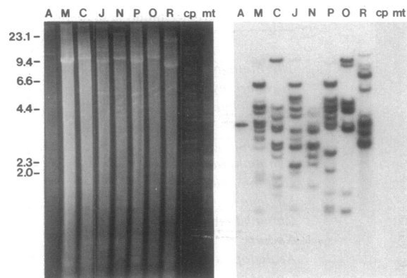
FIG. 5. tufA is a multicopy gene in all Brassicaceae except Arabidopsis . One microgram of ncDNA from Arabidopsis thaliana (A) and 10 \mu g of ncDNAs from Brassica campestris (M), B. carinata (C), B. juncea (J), B. nigra (N), B. napus (P), B. oleracea (O), and Raphanus sativus (R) was digested with Hind III, whereas 100 ng each of B. nigra cpDNA (cp) and mitochondrial DNA (mt) were digested with Eco RI. DNAs were fractionated on a 0.9% agarose gel (Left), blotted onto a nylon filter, and hybridized (Right) with a gel-isolated gene-internal fragment of the Arabidopsis tufA (940-bp Nco I- Stu I). Sizes in kb of Hind III fragments are indicated on the left.
