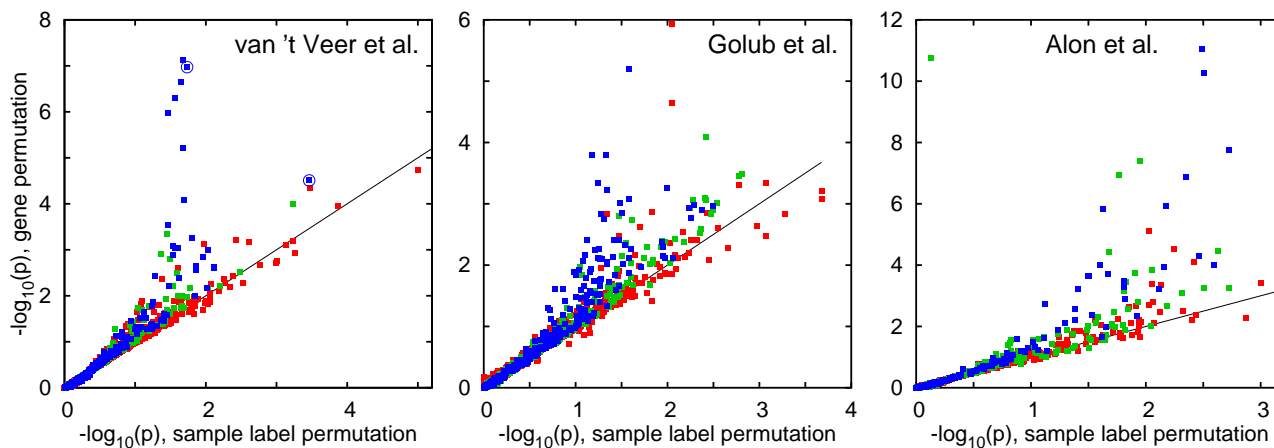
Figure 1 Comparing null hypotheses. Comparison of p -values obtained by sample label permutations and gene permutations, using the data set of van't Veer et al. [13] (left), Golub et al. [11] (middle), and Alon et al. [20] (right). Sample label permutation results were obtained with 100,000 permutations for the van't Veer et al. data set and with 10,000 permutations for the other data sets. Gene permutation results were calculated as described in Methods. Red, green and blue colours represent categories with 1 to 5, 6 to 20, and over 20 genes, respectively. Encircled boxes in the left figure represent the categories "M phase" and "carboxylic acid metabolism", which are further discussed in the text.
