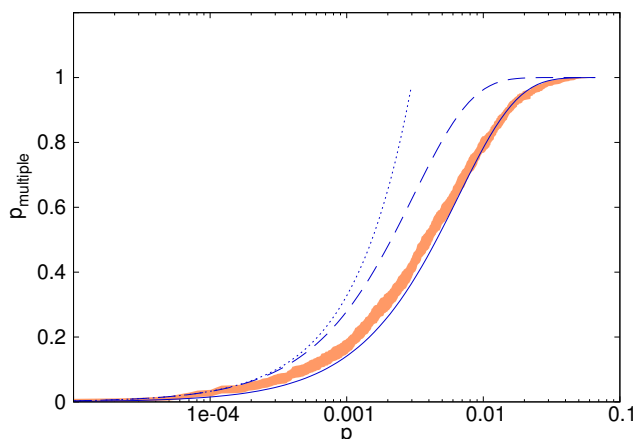
Figure 3 Fitting an effective number of independent categories. The multiple category p -value, p_{\text{multiple}} , versus p -value for the data set of van 't Veer et al. [13], using 327 large Gene Ontology categories with more than 20 genes. The yellow band shows 95% confidence interval of sample label permutation results, based on 1000 random lists, and the blue curves show the results of Equation (1), with the fitted N_{\text{eff}} = 152 (solid line), the total number of categories N = 327 (dashed line), and also the Bonferroni correction (dotted line).
