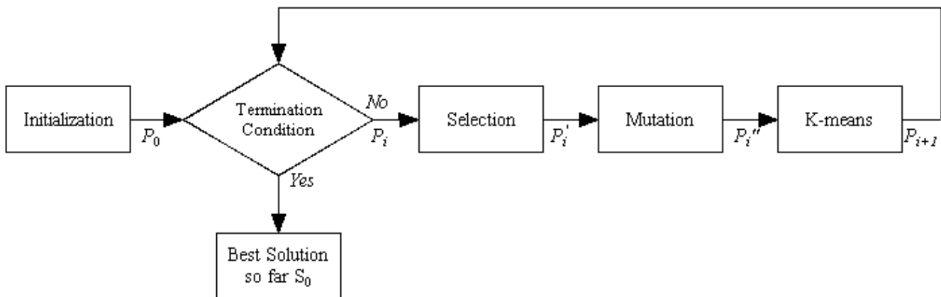
Figure 1 The flowchart of IGKA algorithm. It starts with the initialization phase, which generates the initial population P_0 . The population in the next generation P_{i+1} is obtained by applying genetic operators on the current population P_i . The evolution takes place until a terminating condition is reached. The selection, the mutation and the K-means operator are sequentially used in IGKA.
