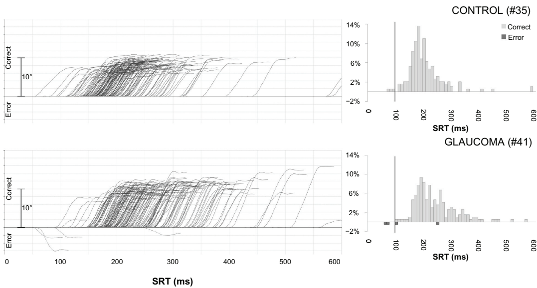
Figure 1 Traces of individual saccades for two subjects (left) and histograms of corresponding reaction times (right). 3 Notes: 3 The left column shows eye position (in degrees) as a function of time (in ms) after the onset of the stimulus. Traces above the x-axis show saccades made in the correct direction for the stimulus, whereas those below show direction errors. Each curve represents a single saccade. The right column shows histograms of reaction times for the two subjects (percentage of total responses on the y-axis, saccade reaction times [SRT] in ms on the x-axis). Light bars above the x-axis represent saccades made in the correct direction, whereas dark bars below the x-axis represent direction error. Data points to the left of the bolded vertical line represent express saccades (saccade reaction times < 100 ms).
