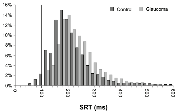
Figure 2 Saccade reaction times (SRT). 3 Notes: 3 Histogram shows the distribution of SRT for each group (percentage of total responses on the y-axis, and in ms on the x-axis). Dark bars represent data from control subjects; light bars represent data from glaucoma patients. Data points to the left of the bolded vertical line at 100 ms represent express saccades.
