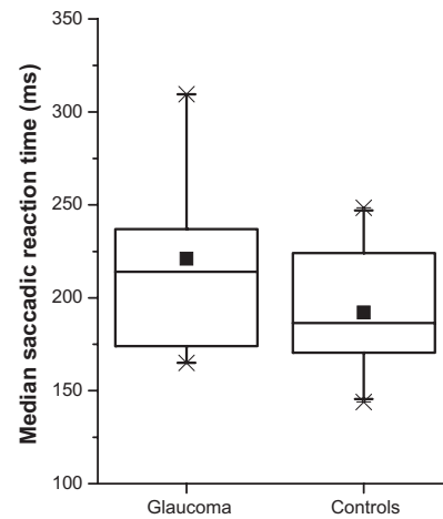
Figure 3 Box plots of median saccadic reaction times per group. 3 Notes: 3 The horizontal bars across the boxes are the medians of the groups; small squares indicate group means. The boxes themselves delineate the 25th percentile to the 75th percentile of each group, the “whiskers” indicate the 5th and 95th percentiles, and the “X”s mark minima and maxima.
