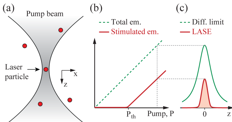
FIG. 1. The principle of LASE microscopy (a) Laser particles excited by a tightly focused optical pump beam. (b) Output energy from a laser particle as a function of pump intensity. The laser output increases steeply at pump energy above the threshold ( P_{th} ). (c) The PSF of laser emission (red line) in comparison to the traditional diffraction-limited PSF of fluorescence detection (green line). Both the resolution and signal-to-background contrast is superior in LASE microscopy.
