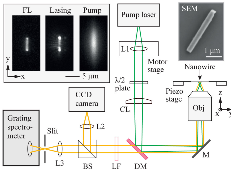
FIG. 3. Schematic of the experimental setup. L1, L2, L3: spherical lenses, \lambda/2 : half-wave plate, CL: cylindrical lens, DM: dichroic mirror, M: mirror, Obj: objective lens (NA=0.8, water immersion), LF: long pass filter, and BS: Beam splitter. SEM: a scanning-electron-microscope image of a typical lead iodide perovskite nanowire. Insets (from left to right): a typical fluorescence image of a perovskite nanowire below threshold, a stimulated emission image above threshold of the nanowire, and a pump beam profile recorded in the CCD camera.
