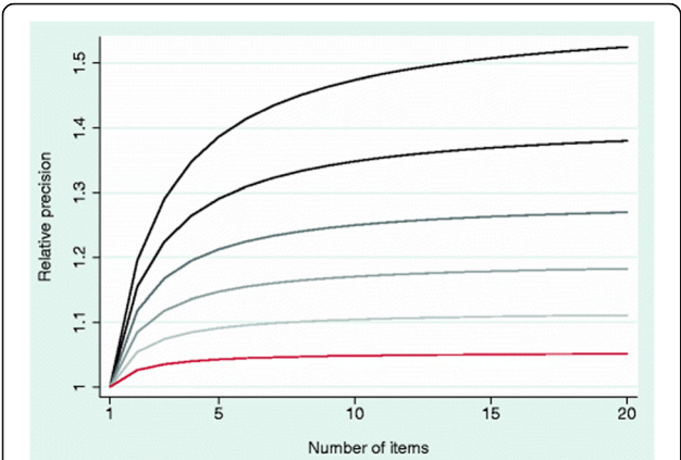
Fig. 2 Relative precision of a domain score by number of items. Shaded lines vary from correlation between items of 0.40 ( black line ) to 0.90 ( red line )
