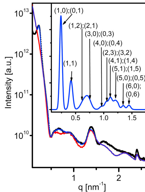
FIGURE 3 Azimuthally integrated scattering intensity as a function of q (the magnitude of the momentum transfer vector, \vec{q} ), from isotropic solution of the SJW1660 strain in 100 mM NaCl (black solid squares). The form factor (red curve) of a flagellar filament was computed using Eqs. 2 and 7 and fitted to experimental data yielding the following essential flagellar structural parameters: filament diameter, D = 23.1 nm; two-turn pitch, p = 5.2 nm; 10.96 flagellin subunits per two-turn pitch; and the radius of the reference point, R = 2.42 nm. The blue curve corresponds to the same form factor when multiplied by the structure factor of a 2D hexagonal phase with a lattice constant, a , of 30.0 nm. The structure factor and its peak indexes are shown in the inset. To see this figure in color, go online.
