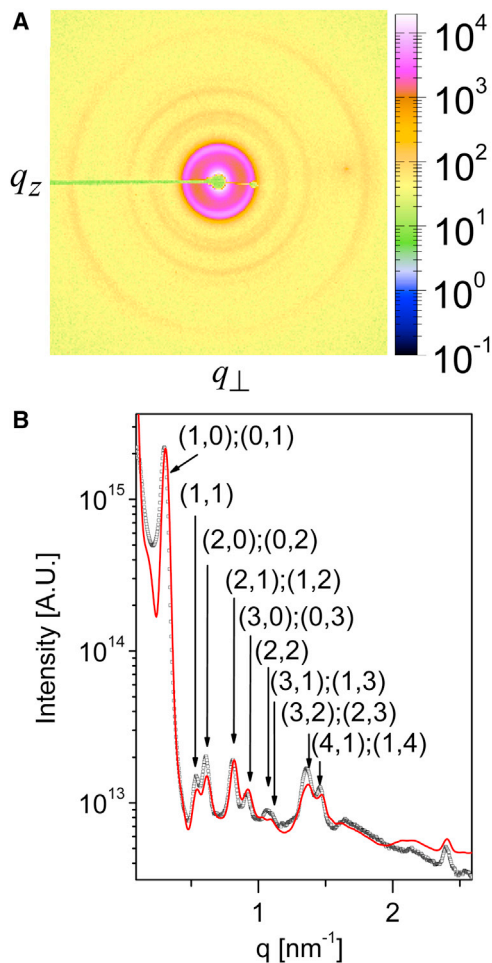
FIGURE 5 Scattering from an isotropic suspension containing bundles of SJW1660 straight flagellar filaments in 100 mM NaCl. The bundles were assembled using a 5 wt % PEG (molecular mass, 20 kDa) concentration, corresponding to an osmotic pressure of 47 kPa (20). (A) Two-dimensional x-ray scattering image. (B) Azimuthally integrated scattering intensity as a function of q . The experimental measurements (black squares) were fitted to our computational hexagonal lattice model (red curve) with a lattice constant of a = 23.5 nm. Good agreement can be seen over a wide q -range in both the location and magnitude of the peaks, whose indexes are indicated in brackets. To see this figure in color, go online.
