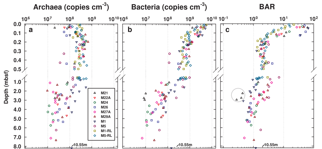
Figure 1. (a) Archaeal and (b) bacterial 16S rRNA gene copy numbers ( \text{copies cm}^{-3} wet sediment) and (c) BARs across a transect of eight stations in Aarhus Bay. The gray circle in (c) marks sediment samples from an organic-poor glacial sand layer at the bottom of M21. The SMTZ was reached at all stations except M21 and M22A, and varied greatly in depth and width (M24: 3.36–4.31 mbsf; M26: 2.04–3.78 mbsf; M27A: 2.62–2.90 mbsf; M29A: 2.20–2.75 mbsf; M1: 1.40–1.60 mbsf; M5: 0.47–0.58 mbsf). Free methane gas was detected at five stations (M26: \geq 7.04 mbsf; M27A: \geq 4.70 mbsf; M29A: \geq 4.45 mbsf; M1: \geq 4.00 mbsf; M5: \geq 1.00 mbsf). Gravity and Rumohr cores were taken from M21, M22A, M24, M26, M27A, M29A, and M5 in May 2010, and from M1 in October 2009. Additional, increased sample-resolution Rumohr cores from M1 (M1-RL) and M5 (M5-RL) were obtained in March 2012.
