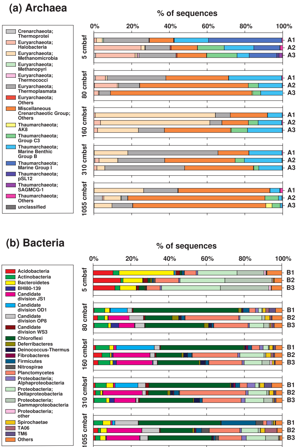
Figure 5. Archaeal and bacterial community compositions in the bioturbation zone (5 cmbsf), the sulfate zone (80 cmbsf), the SMTZ (160 cmbsf), the shallow methane zone (310 cmbsf), and in a freshwater peat layer within the deep methane zone (1055 cmbsf) at M1. Archaeal 16S gene libraries were produced using the primer pairs A1 (Arc806F - Arc958R), A2 (Arc806F - Arc915Rmod), and A3 (Arc915Fmod - Arc1059R), while the bacterial libraries were produced using the primer pairs B1 (Bac8F - Bac338Rabc), B2 (Bac806F_mod2 - Bac908R), and B3 (Bac908F - Bac1075R). Operational Taxonomic Units (OTUs; 97% cutoff) were assigned to class level for Archaea and to phylum level for Bacteria using Mothur, based on an alignment of amplicons to the 16S rRNA reference sequences in SILVA Release 119. See Supplementary Methods for more information.
