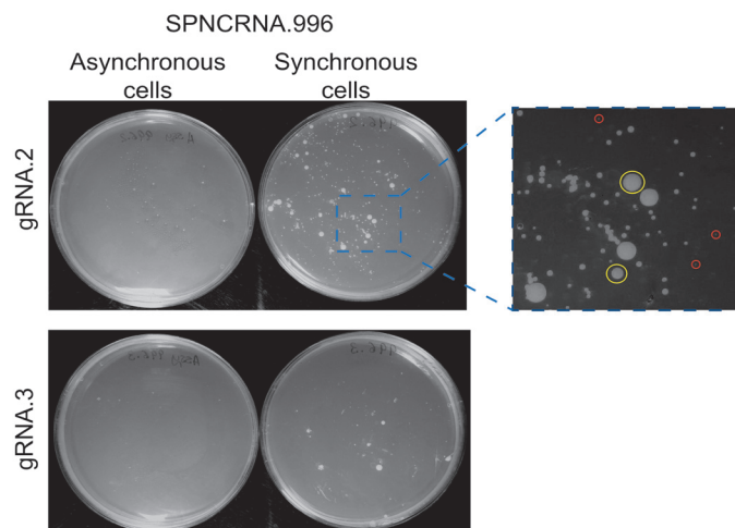
Figure 5. Improved transformation using G1-synchronized, cryopreserved cells. Wild-type cells were cultured in EMM medium and either subjected to nitrogen starvation for 2 hrs (synchronous) or maintained on normal EMM medium (asynchronous) at 25°C. The same number of cells were then made competent and frozen for synchronous and asynchronous cultures. Cryopreserved synchronous and asynchronous cells were transformed with the same amount of DNA for two different sgRNAs, as indicated at top and left. Cells were incubated at 32°C for 4 days, revealing a greatly increased transformation efficiency of the synchronous cells, with no colonies present for unsynchronized cells. Transformation of synchronous cells consistently resulted in 3-fold to over 1000-fold higher numbers of colonies than transformation of asynchronous cells. The enlarged image indicates the smallest colonies that are much more likely to contain successful deletions (red circles) than the large colonies (yellow circles).
