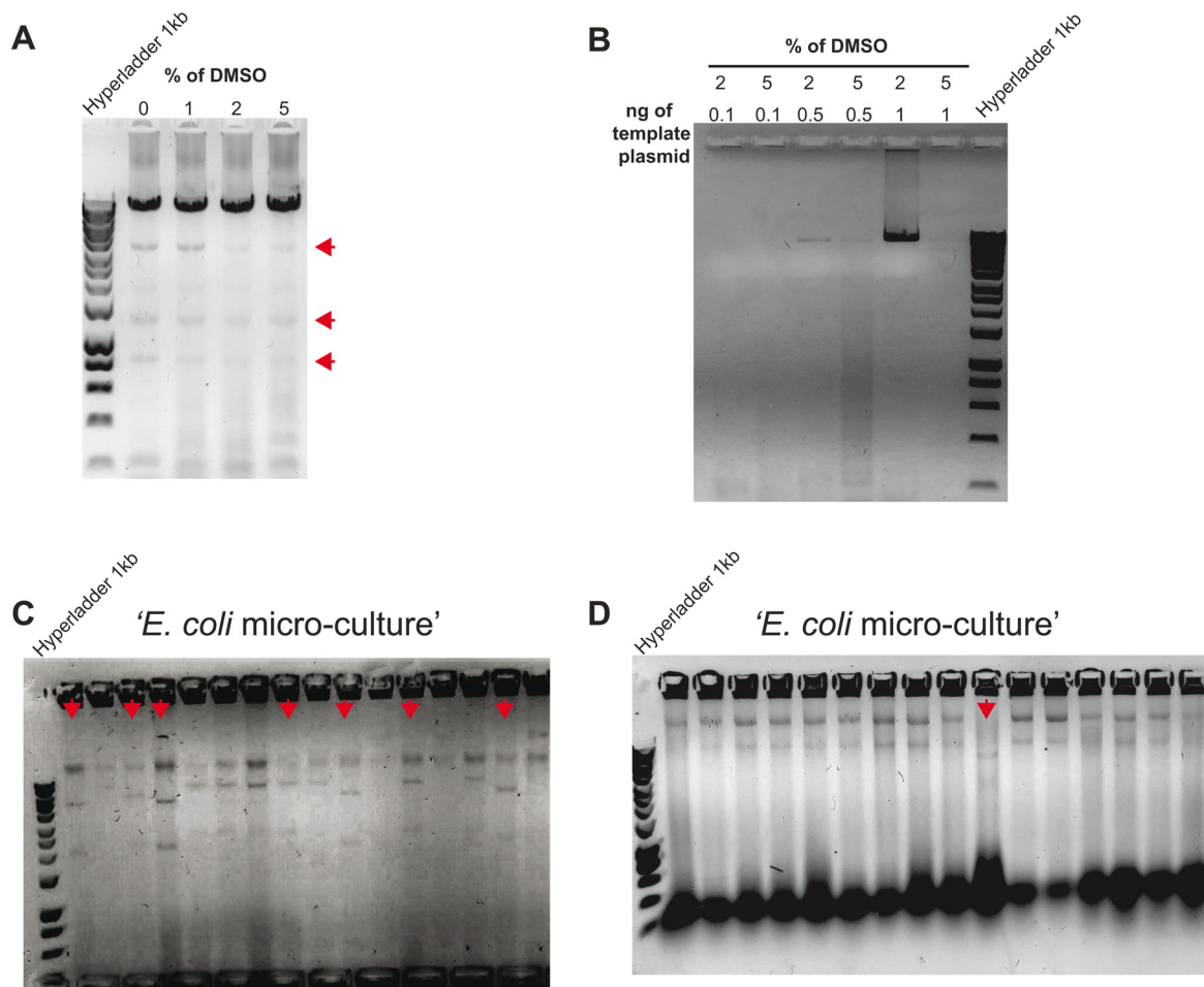
Figure 7. PCR cloning of sgRNA into pMZ379 plasmid and 'E. coli micro cultures'. (A) Gel of non-optimized PCR reactions for sgRNA cloning. Red arrows indicate shorter, unspecific products that need to be removed to avoid faulty plasmids. (B) As in (A), but with optimized PCR reaction which eliminates unspecific products (see protocol for details). (C) Gel of sgRNA-pMZ379 plasmid using non-optimized PCR reactions for sgRNA cloning. Each well contains DNA from different colony of same transformation. Red arrows indicate faulty cloning reactions containing plasmids of different sizes. (D) As in (C), but with optimized PCR reaction used for cloning which largely prevents faulty cloning reactions.
