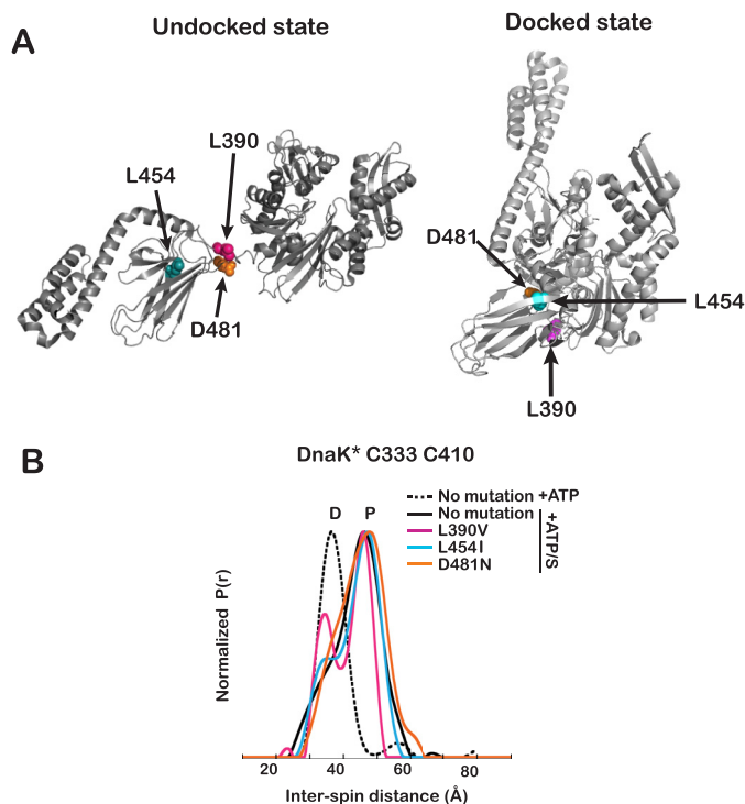
Figure 5. Impact of mutations that modulate the stability of the interdomain interface. A , mutated residues represented as spheres in the structures of DnaK in the undocked (PDB entry 2KH0) and docked (PDB entry 4B9Q) states. B , interspin distance distributions for spin labels on ATP/substrate-bound DnaK* Cys 333 -Cys 410 carrying mutations that stabilize (L390V and L454I) or destabilize (D481N) the interdomain interface. Labeling of the peaks is as in Fig. 3. Data are shown for DnaK* Cys 333 -Cys 410 without the interface mutations for comparison (black lines). Distance distributions for each mutant are shown in magenta for L390V, cyan for L454I, and orange for D481N.
