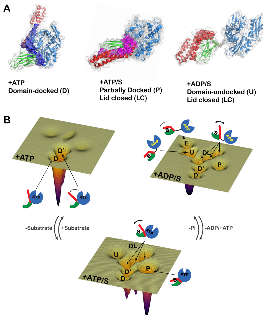
Figure 6. A , schematic representation of the allosterically active state. Shown is a model of the allosterically active state, where the pink spheres represent the interdomain interface formed between NBD and the linker, and between the \alpha and \beta subdomains, when ATP and substrate are bound. The backbone of DnaK has been colored as in Fig. 1A. B , schematic representation of the allosteric energy landscape of DnaK under different ligand-bound conditions. The conformations of DnaK under all nucleotide and substrate conditions detected by IMMS and DEER are represented by schematics on an energy landscape. Each energy landscape contains all of the conformations present in the ensemble that were detected by DEER and IMMS. The depth of each conformational energy well is proportional to the relative abundance based on the DEER measurements.
