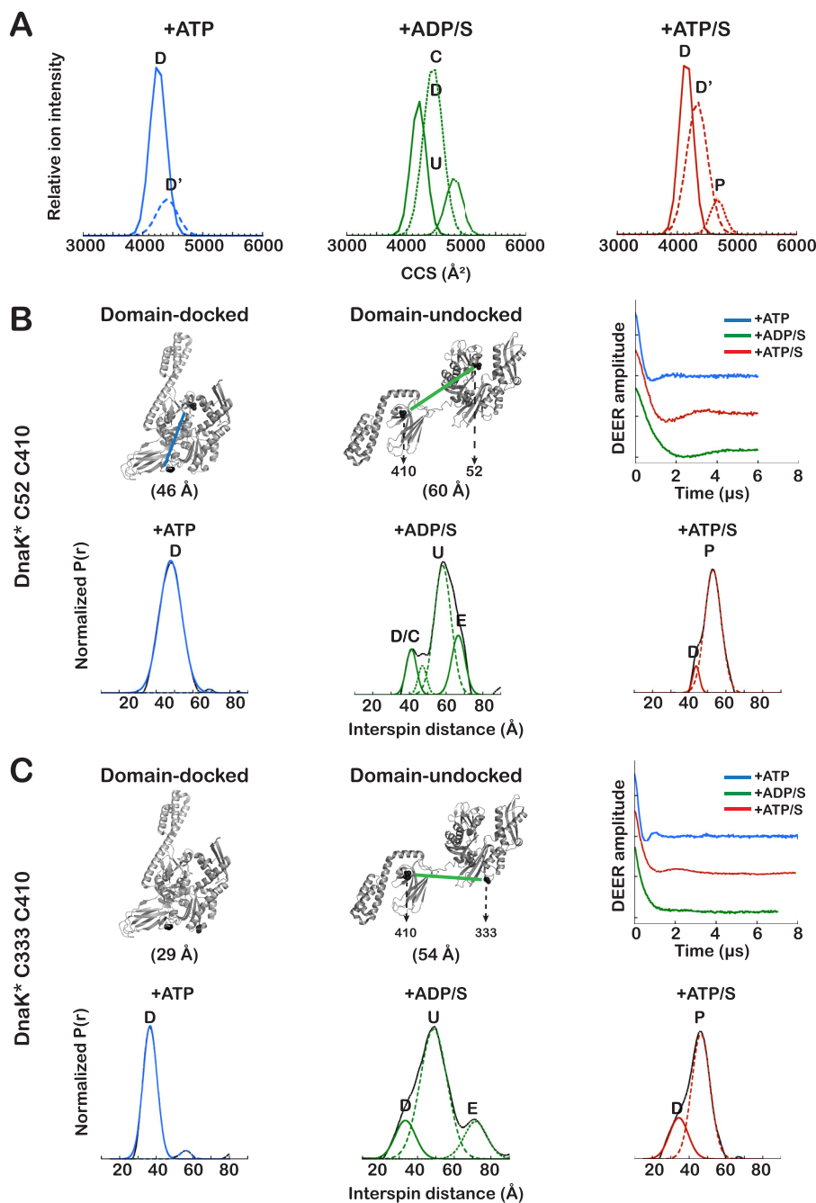
Figure 2. The conformational ensembles of DnaK deduced from IMMS and DEER measurements. A , CCS distributions are shown for all ligand-bound forms of DnaK for ion +17, because this ion is populated under all ligand-bound conditions (ATDs for some ions are shown in supplemental Fig. S1). ATDs for all ions were fit to Gaussian components, as described under “Experimental procedures,” and for each component, the CCS was calculated and used to convert the x axis to CCS (Å 2 ). The components of the same ion are indicated as docked ( D ), domain-docked with detached \alpha -helical lid ( D' ), domain-undocked with domains close ( C ), undocked ( U ), or partially docked ( P ). B and C , left, estimated distance between spins in DnaK* Cys 52 -Cys 410 and DnaK* Cys 333 -Cys 410 , respectively, based on C \beta -C \beta distance in PDB 2KHO and 4B9Q. The estimated distances do not consider the spin-label side chains. Right, baseline-subtracted and normalized data showing time evolution of the interspin coupling. Bottom panels, interspin distance distributions for spin labels on DnaK* in the indicated ligand-bound states. Solid lines, experimental data; dotted lines, fitted Gaussian components. Blue, ATP-bound; green, ADP/substrate-bound; red, ATP/substrate-bound.
