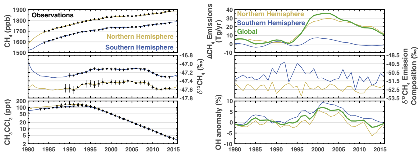
Fig. 2. Most likely solution. Left column shows observed (black triangles) and modeled (solid lines) concentrations of atmospheric CH 4 (Top), \delta^{13}\text{CH}_4 (Middle), and methyl chloroform (Bottom). The Northern Hemisphere is yellow and the Southern Hemisphere is blue. Right column shows the methane emissions (plotted as a deviation from the constant prior emissions; Top), the isotopic composition of the methane emissions (Middle), and the OH anomaly relative to a global mean concentration of 1 \times 10^6 molecules (molec)/cm 3 (Bottom).
