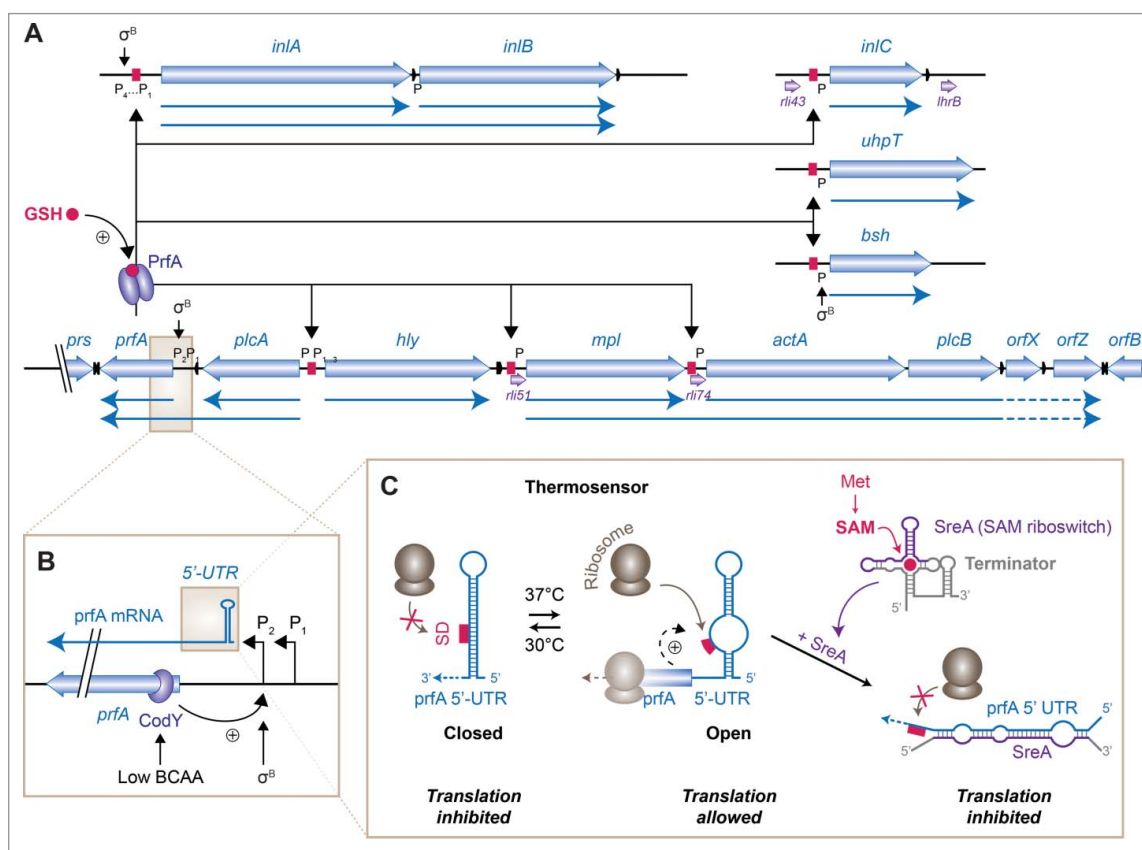
Figure 1. The PrfA regulon and its multiple control mechanisms. (A) Diagram of the main virulence cluster in L. monocytogenes and other PrfA-dependent genes, inspired from Kreft and Vázquez-Boland and de las Heras et al. 9,18 Open reading frames (ORF) are highlighted in thick blue arrows, small RNAs in purple, terminators in black. The main transcriptional units are displayed with plain blue arrows. PrfA binding sites are boxed in magenta. Positive or negative regulators are shown. P, promoter; GSH, glutathione. (B) Transcriptional control of prfA . In addition to \sigma^B -dependent regulation, transcription is enhanced by binding of CodY in the coding sequence, in response to low availability of branched-chain amino-acids (BCAA). UTR, untranslated region. (C) Control of prfA translation initiation, adapted from Cossart and Lebreton. 103 At 30°C, the Shine-Dalgarno (SD) sequence of prfA mRNA is masked from ribosomes by a closed stem-loop structure. At 37°C, a change in the conformation of the 5'-UTR liberates the SD and allows translation initiation. Binding of ribosomes to the SD is further stabilised by the 20 first codons of the ORF. The SreA small RNA, which is the product of a S-adenosylmethionine (SAM) riboswitch, can also base-pair with prfA 5'-UTR and block access of ribosomes to the SD sequence.
