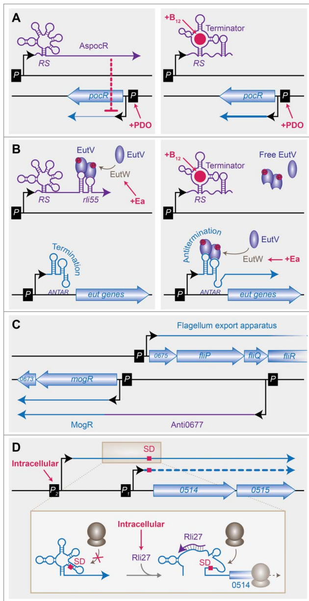
Figure 2. Novel RNA-mediated regulations of L. monocytogenes gene expression. (A) Control of AspocR by a B 12 riboswitch, adapted from Cossart and Lebreton. 103 (Left) In absence of B 12 , full-length AspocR is produced and inhibits pocR expression. (Right) In presence of B 12 , the transcription of AspocR is terminated prematurely by the B 12 riboswitch (RS), and transcription of pocR is allowed, provided that propanediol (PDO) is also present in the medium. (B) Sequestration of an antiterminator by a B 12 riboswitch, inspired from Mellin et al. 75 In presence of Ethanolamine (Ea), the antiterminator EutV is phosphorylated by EutW and activated. (Left) In absence of B 12 , full-length Rli55 is produced and sequesters active EutV. The transcription of eut genes is prevented by early termination at the ANTAR elements. (Right) In presence of B 12 , the transcription of Rli55 is terminated prematurely by the B 12 riboswitch. Free phosphorylated EutV dimers can then bind the ANTAR element and mediate antitermination, allowing the expression of eut genes. (C) The mogR-flj locus exclusion, adapted from Cossart and Lebreton. 103 mogR is encompassed by 2 transcripts. In the longest one, the 5'-UTR of upstream of MogR coding sequence also acts as an antisense RNA, Anti0677, overlapping the flj operon. The two divergent transcriptional units encode proteins of opposite functions: MogR is a transcriptional repressor of flagellum genes, whereas Fli proteins participate in the flagellum export apparatus. (D) Rli27 allows the intracellular-specific translation of an alternative transcript, inspired from Quereda et al. 94 Extracellular bacteria express mainly lmo0514-lmo0515 from the constitutive P1 promoter. An alternative, long mRNA is produced in low amounts from P2, but ribosomes cannot access the Shine-Dalgarno sequence (SD). In cells, the P2 promoter is activated, and Rli27 is expressed. Base-pairing of Rli27 with the 5'-UTR of the long transcript allows ribosome binding and translation to proceed.
