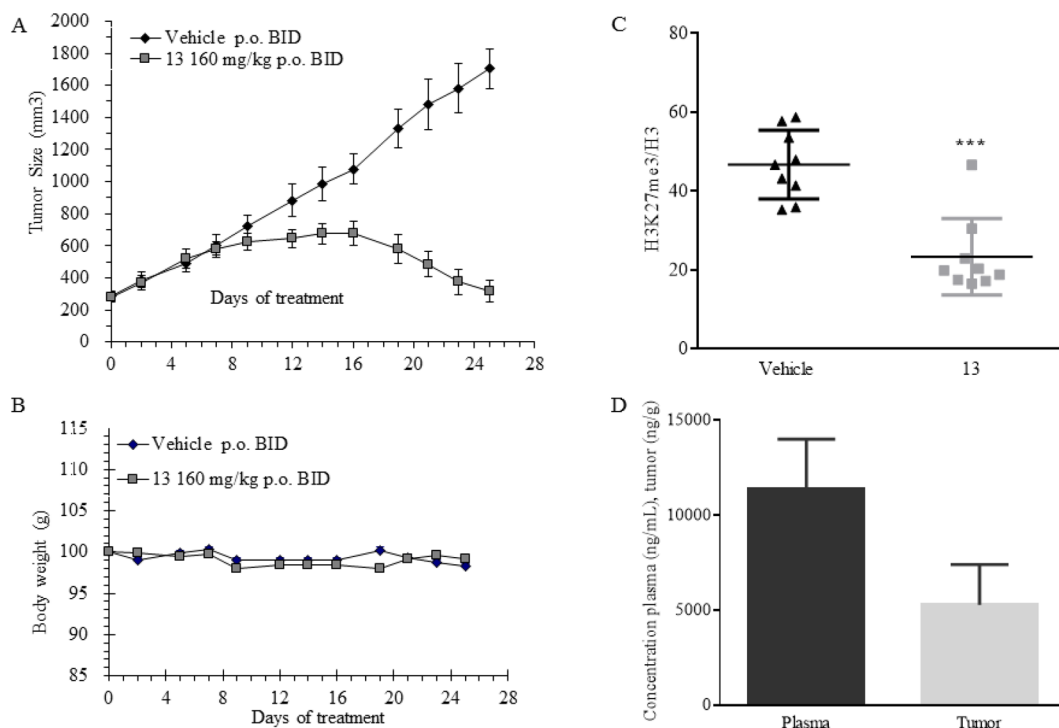
Figure 6. Tumor xenograft with 13. (A) Effect of dosing analogue 13 at 160 mpk BID for 25 days on KARPAS-422 tumor growth in mouse xenograft. (B) Corresponding body weight change during the course of the study. (C) Pharmacodynamic effect of 13 on reduction of H3K27me3 normalized to total H3. (D) Analysis of plasma and tumor concentrations of 13 at 1 h post last dose on day 25.
