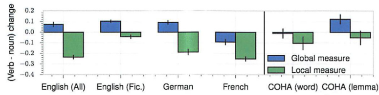
Figure 2. The global measure is more sensitive to semantic changes in verbs while the local neighborhood measure is more sensitive to noun changes
