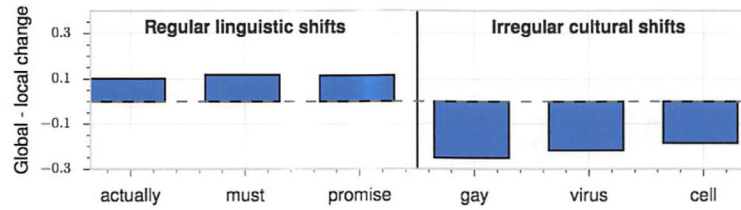
Figure 3. The global measure captures classic examples of linguistic drift while the local measure captures example cultural shifts
