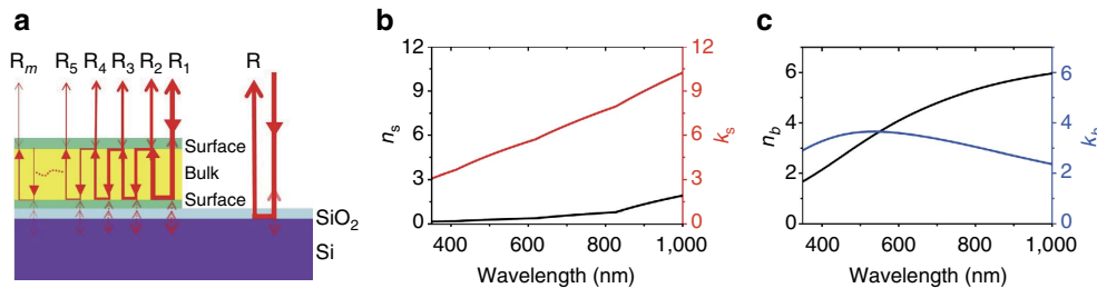
Figure 2 | Physical mechanism of the Sb_2Te_3 thin film cavity. (a) Diagram of internal light multiple reflections in the resonant cavity of the Sb_2Te_3 thin film. The semi-transparent arrows indicate interface reflections. (b) The surface refractive index n and extinction coefficient k curves of the Sb_2Te_3 thin film as a function of wavelengths. (c) The bulk refractive index n and extinction coefficient k curves of the Sb_2Te_3 thin film as a function of wavelengths.
