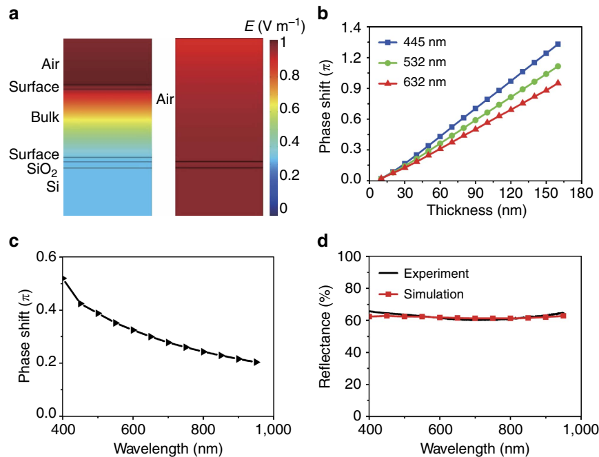
Figure 3 | Numerical simulations of electromagnetic fields and phase shift. (a) Simulated electromagnetic field distributions in the Sb_2Te_3 thin film cavity and the SiO_2/Si substrate under illumination with 632 nm light. (b) Simulated phase shift between the Sb_2Te_3 film and the SiO_2/Si substrate as a function of the film thickness at different wavelengths. (c) Simulated phase shift between the 60 nm Sb_2Te_3 film and the SiO_2/Si substrate as a function of wavelength. (d) Simulated and experimental reflectance of 60 nm Sb_2Te_3 thin films as a function of wavelength. The simulation shows good agreement with experiments.
