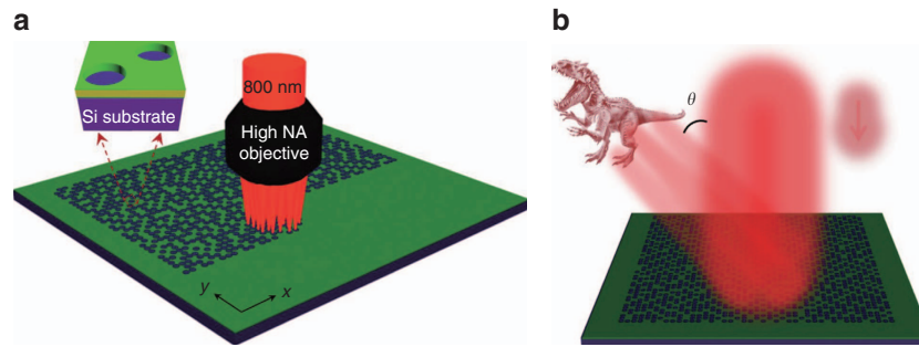
Figure 1 | Nanofabrication of the binary hologram and holographic imaging procedures. (a) Nanofabrication process of a nanometric Sb_2Te_3 hologram using the direct laser write system. The upper inset displays the ablated pixels in the topological insulator thin film. (b) Holographic imaging procedure of a nanometric Sb_2Te_3 hologram using a continuous wavelaser beam. \theta is the projection angle of the holographic image. Note: this figure is not included under the article CC BY licence; Indominus Rex image is reproduced with permission from the publisher Comingsoon.net and copyright owner Universal Studios.
