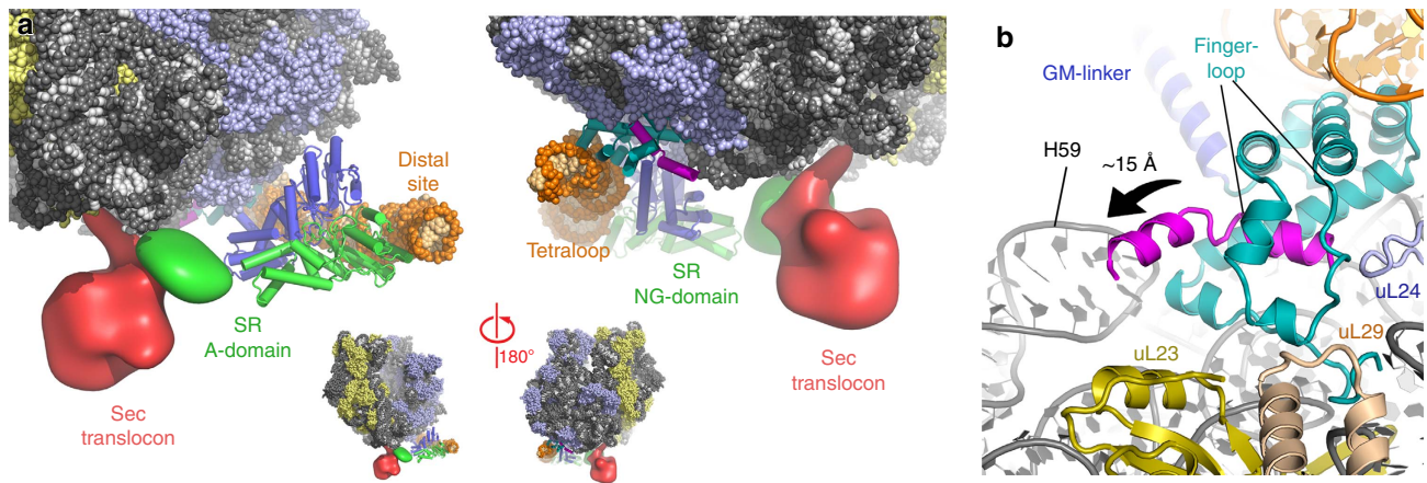
Figure 3 | Localization of the translocon and the signal sequence in the quaternary complex. (a) Position of the Sec translocon on the RNC in close proximity to the extending signal sequence, bound to the SRP M domain, and the A-domain of SR. (b) Close-up views of the interactions between the M-domain fingerloop of the SRP protein and the ribosomal protein uL29 (wheat), where the signal sequence extends three helical turns outwards from the M-domain.
