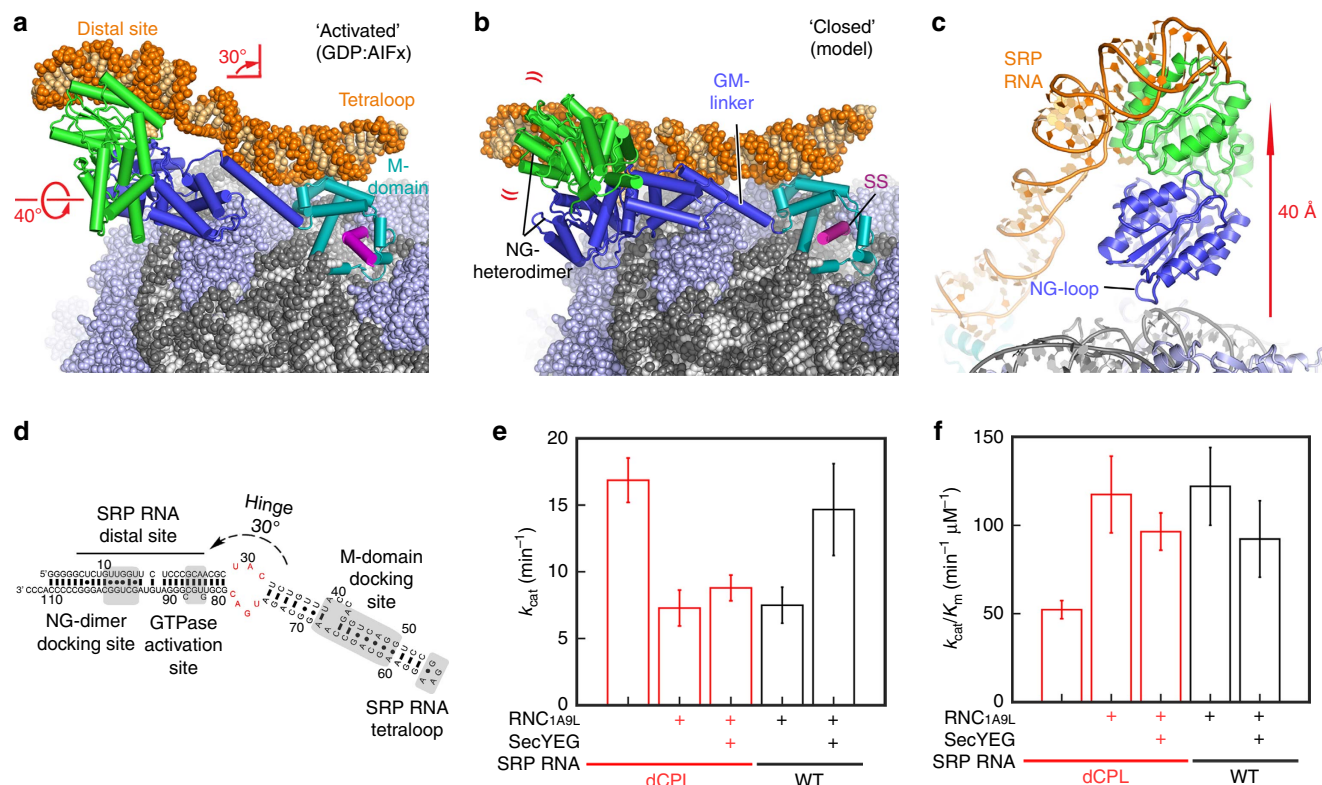
Figure 2 | Conformation of the SRP-SR ribosome complex in the 'activated' state. (a) Atomic model of the SRP-SR complex bound to the RNC in the 'activated' state. The curved arrows demonstrate a kink upwards by 30° and an anti-clockwise untwisting by 40° in the SRP RNA, compared to (b). (b) Composite model of the NG heterodimer as seen in the crystal structure of the isolated SRP-SR complex (PDB:2XXA), here shown docked on the ribosome based on the known position of the M-domain (PDB:5GAG). (c) Close-up view of the interaction between H100 of the rRNA and the NG loop of SRP displayed as cartoon. (d) Secondary structure of the E. coli SRP RNA: the tetraloop, M-domain, GTPase activation and NG heterodimer docking sites are highlighted in grey. The SRP RNA C-loop region, where the 30° kink in the RNA is observed, is shown in red. (e) Effect of the C-loop mutation of the SRP RNA on the SRP-SR GTPase hydrolysis rate ( k_{cat} ) in the presence and the absence of the RNC 1A9L -85 and the Sec translocon. (f) Effect of the C-loop mutation on the assembly rate constant of the SRP-SR complex ( k_{cat}/K_m ) with or without RNC and SecYEG present.
