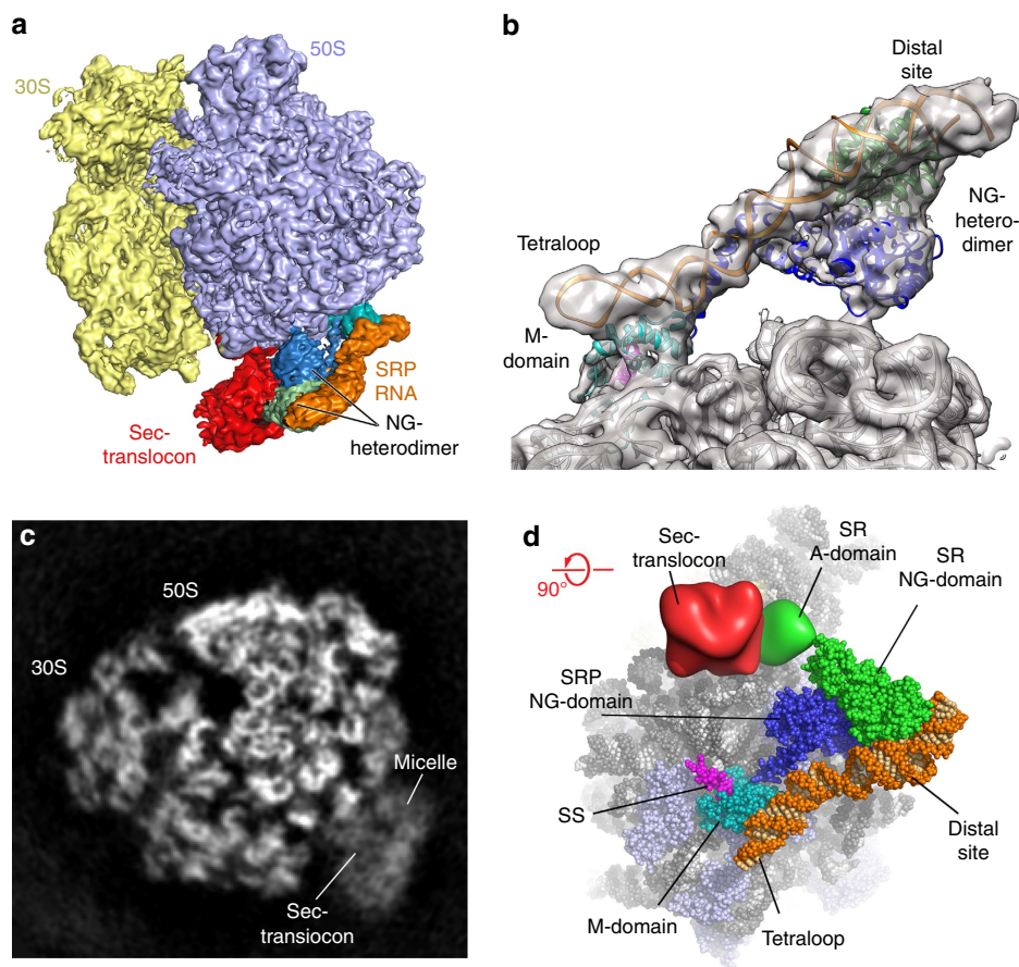
Figure 1 | Structure of the SRP-SR-Sec translocon and RNC quaternary complex. (a) Cryo-EM reconstruction of the SRP-SR-Sec translocon with RNC quaternary complex at 4.8 Å (SRP RNA—orange, SRP protein M domain—cyan, SRP protein NG domain—dark blue, SR—green, translocon—red). (b) Representative view of the conformation of the SRP RNA and the SRP-SR NG heterodimer in the 'activated' state, with overlaid EM density filtered to 5 Å. (c) Cross-section of the unsharpened EM-density map of the quaternary complex showing secondary structural elements of the Sec translocon within the unstructured detergent micelle. (d) The structure of the complex shown towards the ribosomal tunnel exit. Structures that were interpreted with atomic coordinates are shown as spheres, whereas, the A domain of the receptor and the Sec translocon are depicted as a surface representation. Signal sequence (SS) is shown in magenta.
