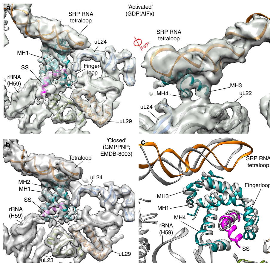
Figure 4 | Conformational state of the M-domain. (a) EM densities of the quaternary complex in the pre-transfer state (this study) with fitted atomic coordinates. (b) EM density of the closed state of the SRP-SR complex solved in the presence of GMPPNP (EMDB:8003, PDB:5GAG), filtered to 5 Å. (c) Overlay the two atomic coordinates to illustrate the conformational change. Atomic coordinates of the M-domain and the signal sequence in the 'closed' state are shown in grey. Colouring scheme is identical to Fig. 1.
