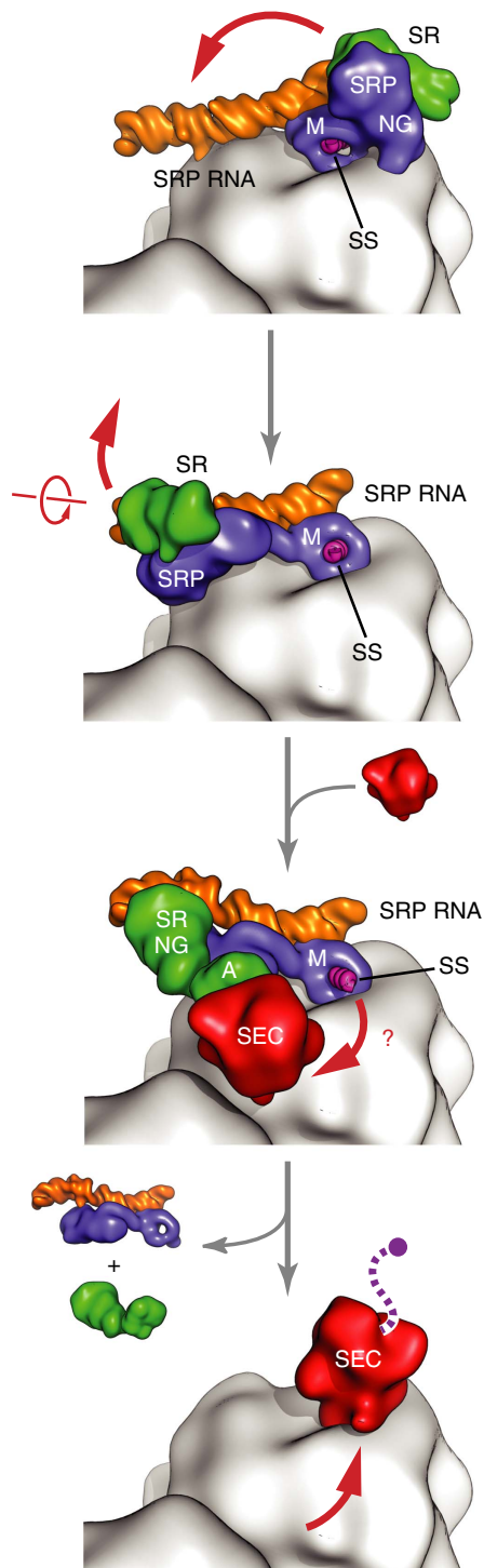
Figure 5 | Proposed cargo handover mechanism of co-translational protein targeting. Schematic of the early, closed and activated/quaternary targeting complexes ending with the RNC in complex with the Sec translocon. Initially the SR binds to the SRP RNC complex at the tetraloop side of the SRP RNA, followed by repositioning and docking of the NG heterodimer to the distal region of SRP RNA. GTPase activation becomes possible upon conformational change in the SRP RNA that accommodates NG heterodimer between the SRP RNA and the ribosomal surface. Signal sequence handover is favored for longer nascent chains that can reach Sec translocon. Sec translocon will then displace the M-domain and SRP from the ribosome exit tunnel to complete the targeting cycle.
