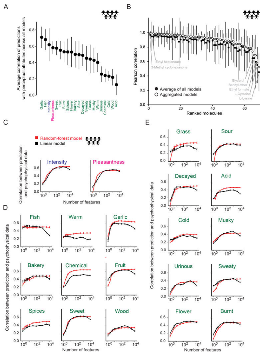
Fig. 3. Predictions of population perception
