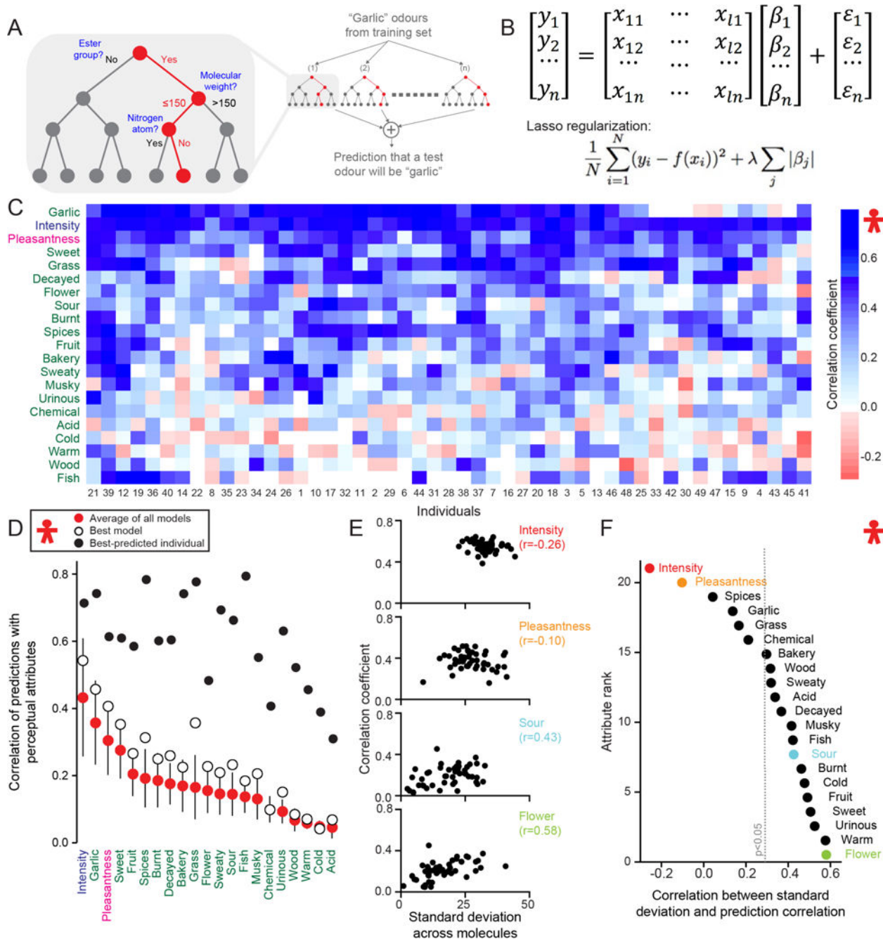
Fig. 2. Predictions of individual perception
