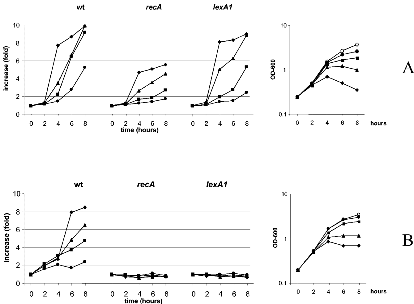
FIG. 2. Effects of the \Delta(\text{sr}L\text{-rec}A)306::\text{Tn}10 and lexA1 genetic backgrounds on the ceftazidime-mediated induction of transcription of the dinB::lacZ fusion. The curves on the left of each panel indicate the transcription levels ( n -fold) between treated and nontreated cultures (calculated by assigning a value of 1 to the transcription level of the nontreated culture at each time point). Concentrations of CAZ (A) and NAL (B) expressed in micrograms per milliliter were as follows: 1 ( \blacklozenge ), 2 ( \blacktriangle ), 4 ( \blacksquare ), and 8 ( \bullet ). The mean values of results from three independent experiments are displayed. The curves on the right of each panel represent the growth curves without and with CAZ or NAL for strain GW1030 (symbols are as described for the transcription levels; \circ indicates the values obtained without CAZ). Curves for recA and lexA1 derivatives are not presented because they are similar to those for strain GW1030. OD-600, optical density at 600 nm; wt, wild type.
