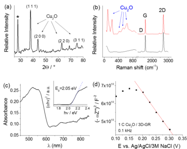
Figure 5. (a) XRD pattern, (b) Raman spectrum (also for the bare 3D-GR sample), (c) Diffuse-reflectance UV-vis spectrum (together with Tauc representation as inset), and (d) Mott-Schottky plot (recorded in 0.1 \text{ M NaAc} solution), of a \text{Cu}_2\text{O}/3\text{D-GR} composite, deposited with 1 \text{ C cm}^{-2} charge density. The diffraction marked with asterisk in (a) corresponds to the graphene substrate.
