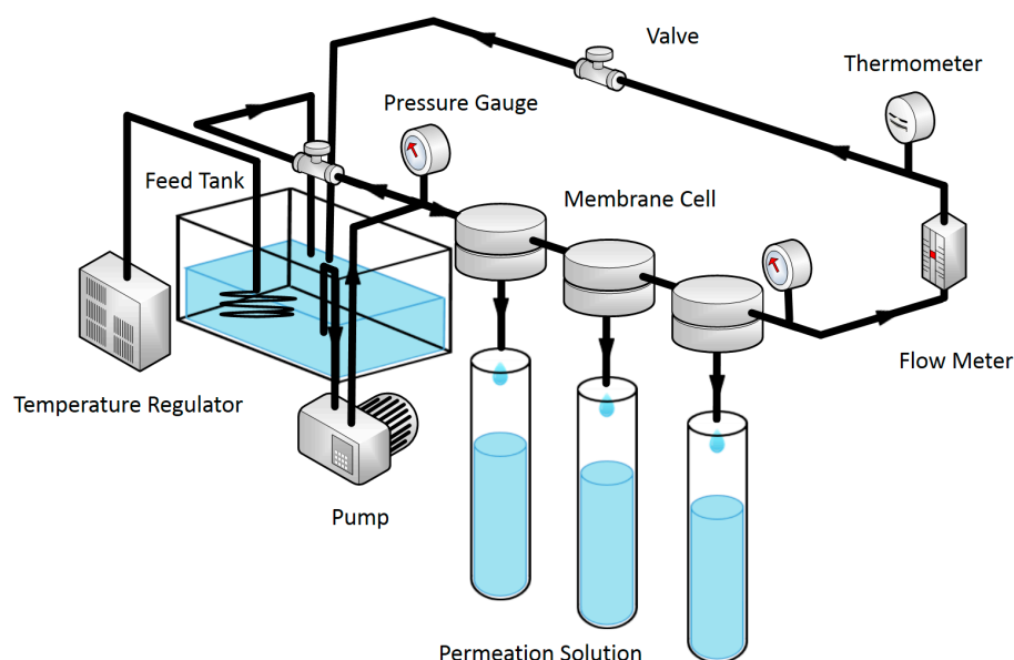
Figure 1. Schematic representation for the membrane performance evaluation instrument.
