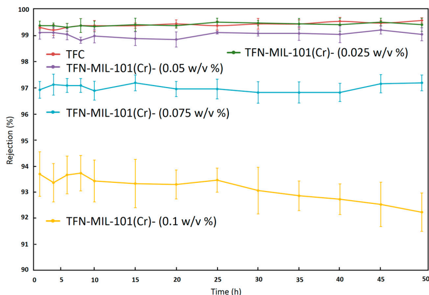
Figure 10. NaCl rejection of TFN-MIL-101 (Cr)-O membranes during 50 h stability test with 2000 ppm NaCl aqueous solution at 16 bar and 25 °C.
