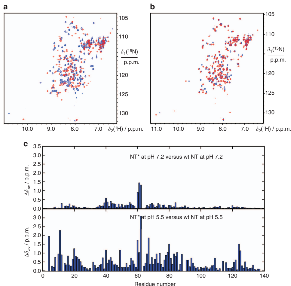
Figure 3 | Comparison of NTwt and NT* using 2D HSQC NMR. (a) Overlay of ^{15}\text{N} - ^1\text{H} HSQC-NMR spectra of \text{NT}_{\text{wt}} (red) and \text{NT}^* (blue) at pH 5.5. (b) Overlay of ^{15}\text{N} - ^1\text{H} HSQC-NMR spectra of \text{NT}_{\text{wt}} (red) and \text{NT}^* (blue) at pH 7.2. (c) Averaged backbone amide ^1\text{H} and ^{15}\text{N} chemical shift differences \Delta\delta_{\text{av}} = \sqrt{(0.1\Delta\delta_{\text{N}})^2 + (\Delta\delta_{\text{H}})^2} between \text{NT}_{\text{wt}} and \text{NT}^* at pH 5.5 and pH 7.2.
