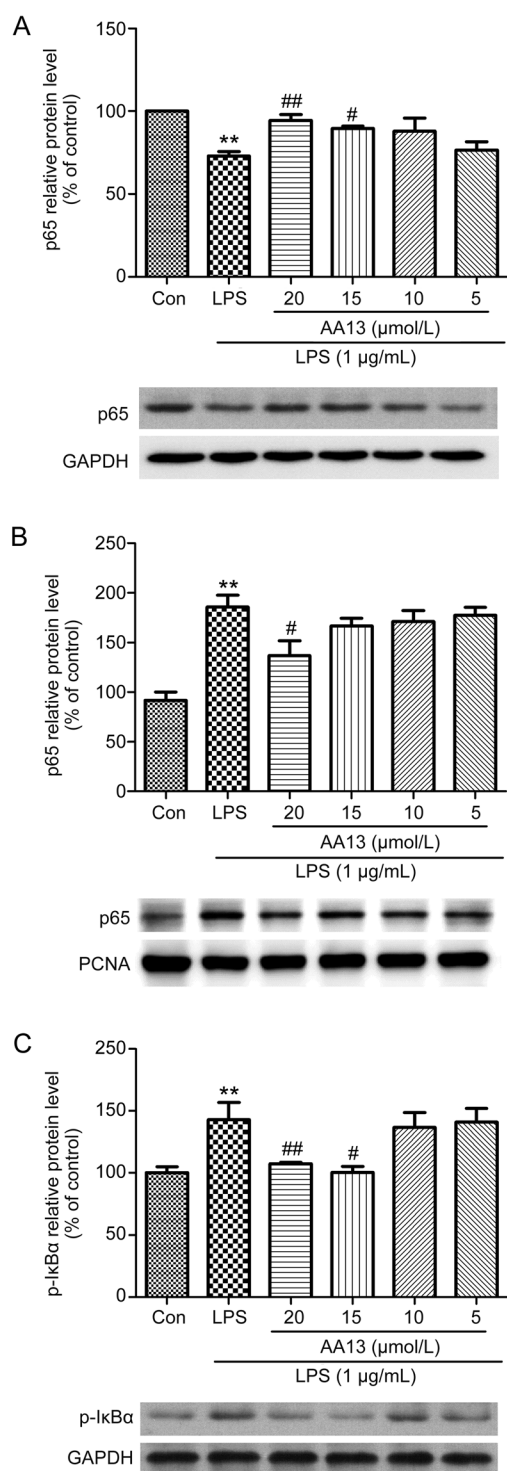
Figure 8. Effect of AA13 on LPS-stimulated NF- \kappa B p65 translocation in RAW264.7 cells ( n=3 for each group). Cells were pretreated with AA13 for 30 min, followed by LPS ( 1 \mu\text{g/mL} ) stimulation for 1 h. Cytoplasmic (A) and nuclear (B) extracts were used to analyse p65 translocation by Western blot. GAPDH and PCNA were used as internal control to cytoplasmic and nuclear fractions. I \kappa B phosphorylation (C) was measured to confirm the NF- \kappa B activation. Mean \pm SEM. n=3 independent experiments. ** P<0.01 vs control group. # P<0.05 , ## P<0.01 vs LPS-stimulated group.
