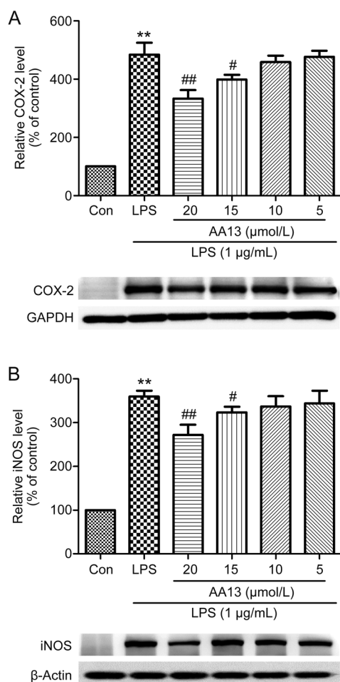
Figure 5. The inhibition effect of AA13 on LPS-stimulated COX-2 and iNOS in RAW264.7 cells ( n=3 for each group). Cells were pretreated with AA13 for 30 min, followed by LPS ( 1 \mu\text{g}/\text{mL} ) stimulation for 1 h. The level of COX-2 (A) and iNOS (B) were determined by Western blot. Mean \pm SEM. n=3 independent experiments. ** P<0.01 vs control group. # P<0.05 , ## P<0.01 vs LPS-stimulated group.
