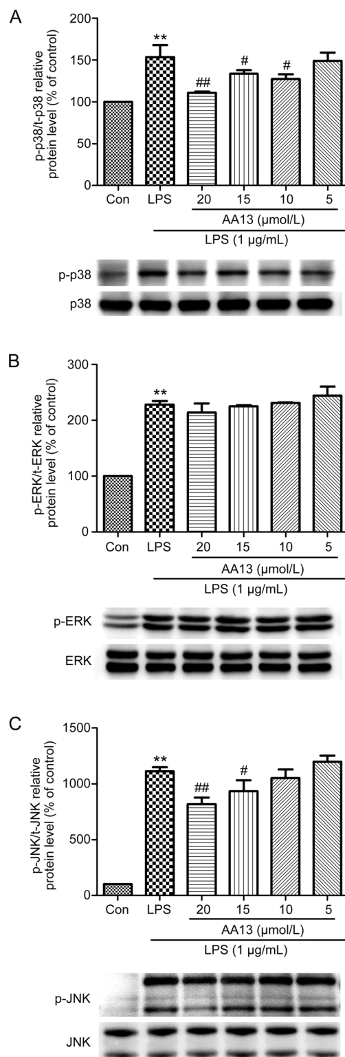
Figure 6. Effect of AA13 on LPS-stimulated MAPKs pathway in RAW264.7 cells ( n=3 for each group). Cells were pretreated with AA13 for 30 min, followed by LPS ( 1 \mu\text{g}/\text{mL} ) stimulation for 1 h. The level of p-p38/p38 (A), p-ERK/ERK (B) and p-JNK/JNK (C) were determined by Western blot. Mean \pm SEM. n=3 independent experiments. ** P<0.01 vs control group. # P<0.05 , ## P<0.01 vs LPS-stimulated group.
