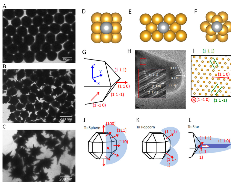
Figure 5. Computational studies on growth mechanisms of IO-Au core-shell nanospheres, nanopopcorns, and nanostars. (A–C) TEM images of IO-Au core-shell nanospheres, nanopopcorns, and nanostars. (D–F) The adsorption of Ag on the Au (100) surface (D), Au (110) surface (E), and Au (111) surface (F). (G) Schematic of the proposed geometry of the tip of the nanostar. (H) HRTEM image of a tip of the nanostar. The inset shows an enlarged view of the lattice, where the position of each atom is visible. (I) The positions of atoms according to the proposed model in (G), which is viewed from the [1-10] direction. (J–L) The growth mechanism of Au nanospheres (J), nanopopcorn (K), and nanostars (L). Reprinted with permission from ref 72. Copyright (2016) American Chemical Society.
