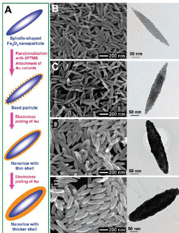
Figure 3. Synthesis of IO-Au core-shell nanorices via an Au-seeded growth method. (A) Schematic of the preparation of IO-Au core-shell nanorices. (B–E) SEM (left) and TEM (right) images of IO-Au core-shell nanorices at different preparation steps. (B) The IO nanorices. (C) Au-seeded IO nanorices. (D) IO-Au core-shell nanorices with thin shells (~13 nm). (E) IO-Au core-shell nanorices with thick shells (~28 nm). Reprinted with permission from ref 80. Copyright (2006) American Chemical Society.
