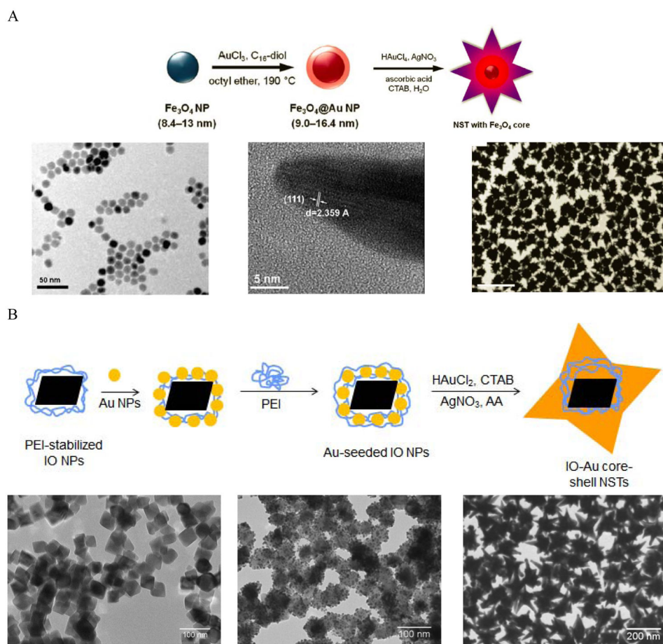
Figure 4. Synthesis of IO-Au core-shell NSTs. (A) Synthesis of IO-Au core-shell NSTs from small IO-Au core-shell nanospheres. (Top) Schematic of the preparation procedure. (Bottom) TEM image of IO NPs (left), HRTEM image of a tip (middle), and TEM image of IO-Au NSTs. Reprinted with permission from ref 82. Copyright (2010) American Chemical Society. (B) Synthesis of IO-Au core-shell NSTs by the Au-seeded growth method. (Top) Schematic of the preparation procedure. (Bottom) TEM images of IO NPs (left), Au-seeded IO NPs (middle) and IO-Au NSTs. Reprinted with permission from ref 72. Copyright (2016) American Chemical Society.
