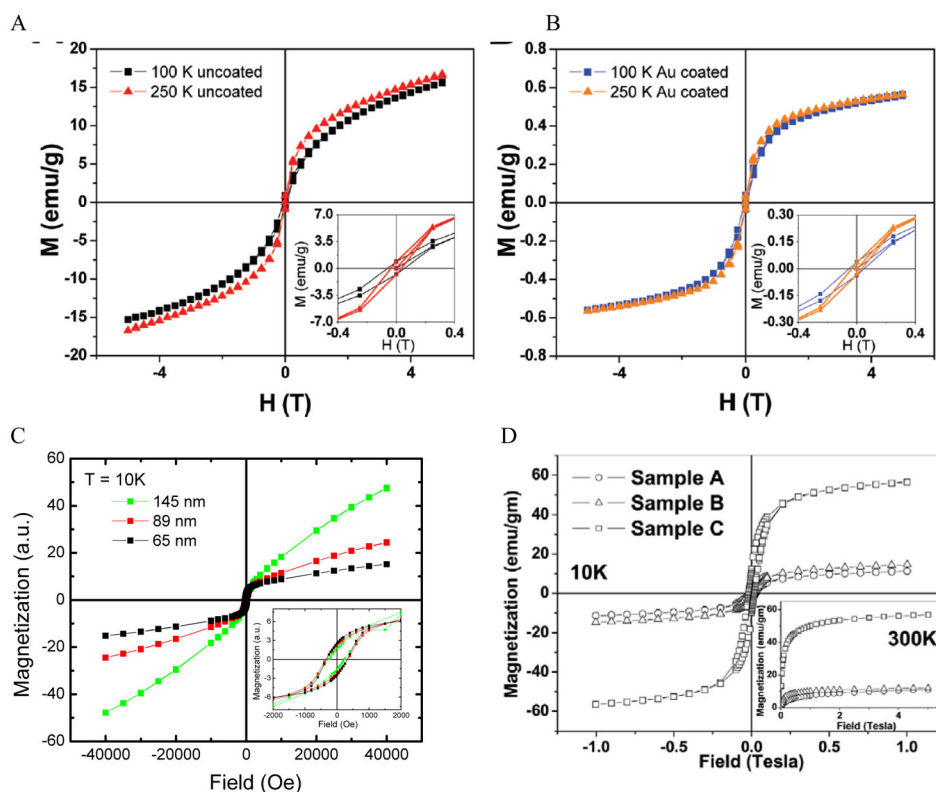
Figure 6. Magnetic properties of IO-Au core-shell NPs. (A–B) Magnetization as a function of applied field at 100 K and 250 K for uncoated and Au coated tetracubic IO NPs. Reprinted with permission from ref 69. Copyright (2009) American Chemical Society. (C) Magnetization as a function of applied field at 10 K for IO-Au core-shell nanopopcorns of three different sizes. Reprinted with permission from ref 72. Copyright (2016) American Chemical Society. (D) Magnetization as a function of applied field at 10 K and 300 K for bare IO NPs (sample A), IO-Au core-shell NPs with low Au (sample B) and high Au (sample C). Reprinted with permission from ref 46. Copyright (2011) American Chemical Society.
