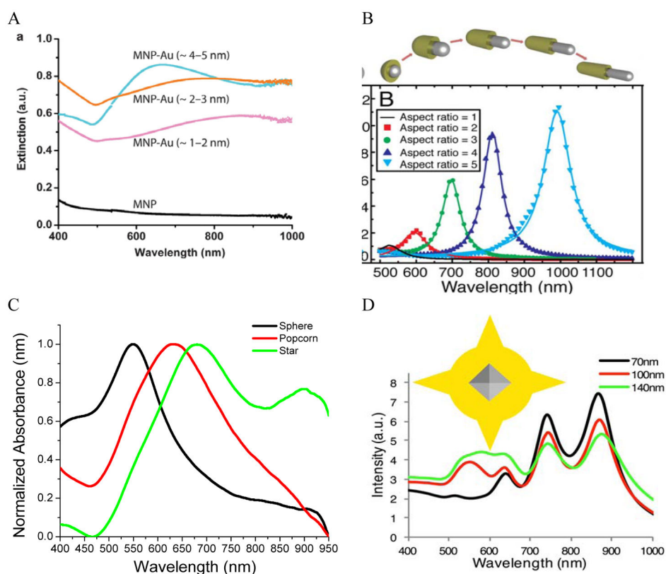
Figure 8. NIR absorbing IO-Au core-shell NPs. (A) Absorption spectra of \text{Fe}_3\text{O}_4 -Au core-shell NPs with different shell thickness. D core = 25 nm. Reprinted by permission from Macmillan Publishers Ltd: [Nature Communications] (ref 44), copyright (2010). Calculated extinction spectra of IO-Au core-shell NRs with different aspect ratios. Reprinted with permission from ref 106. Copyright (2011) Elsevier. (C) Absorption spectra of \text{Fe}_3\text{O}_4 -Au core-shell NPs with different shapes. The \text{Fe}_3\text{O}_4 core is octahedral with an edge length of 35 nm. Reprinted with permission from ref 72. Copyright (2016) American Chemical Society. (D) Calculated extinction spectra of IO-Au core-shell NSTs with different base size. The \text{Fe}_3\text{O}_4 core is octahedral with an edge length of 35 nm. Reprinted with permission from ref 72. Copyright (2016) American Chemical Society.
