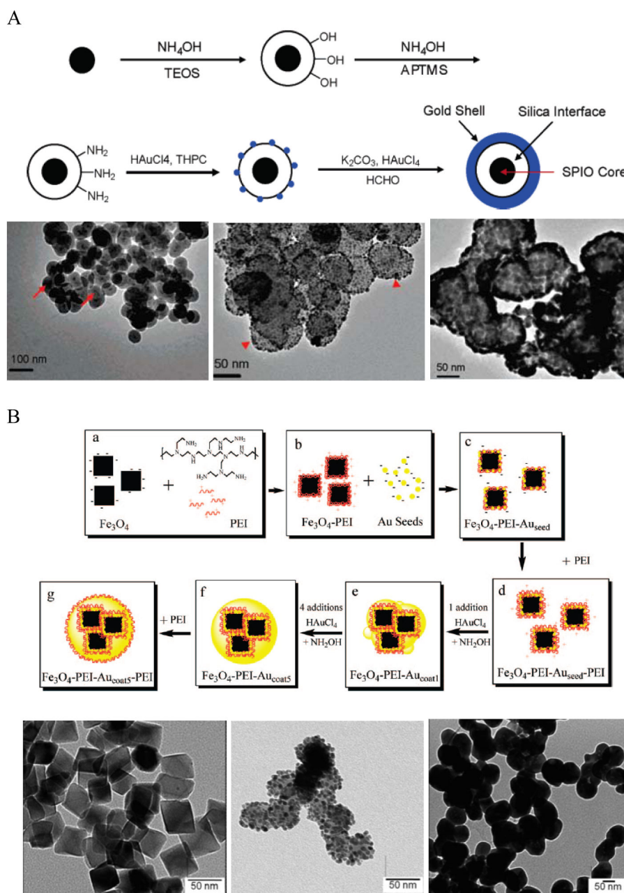
Figure 2. Synthesis of IO-Au core-shell NPs via Au-seeded growth methods. (A) APTMS and (B) PEI are used as the anchor agent for the adsorption of Au seeds on IO NPs. (A) is reprinted with permission from ref 23. Copyright (2007) American Chemical Society. (B) is reprinted with permission from ref 71. Copyright (2009) American Chemical Society.
