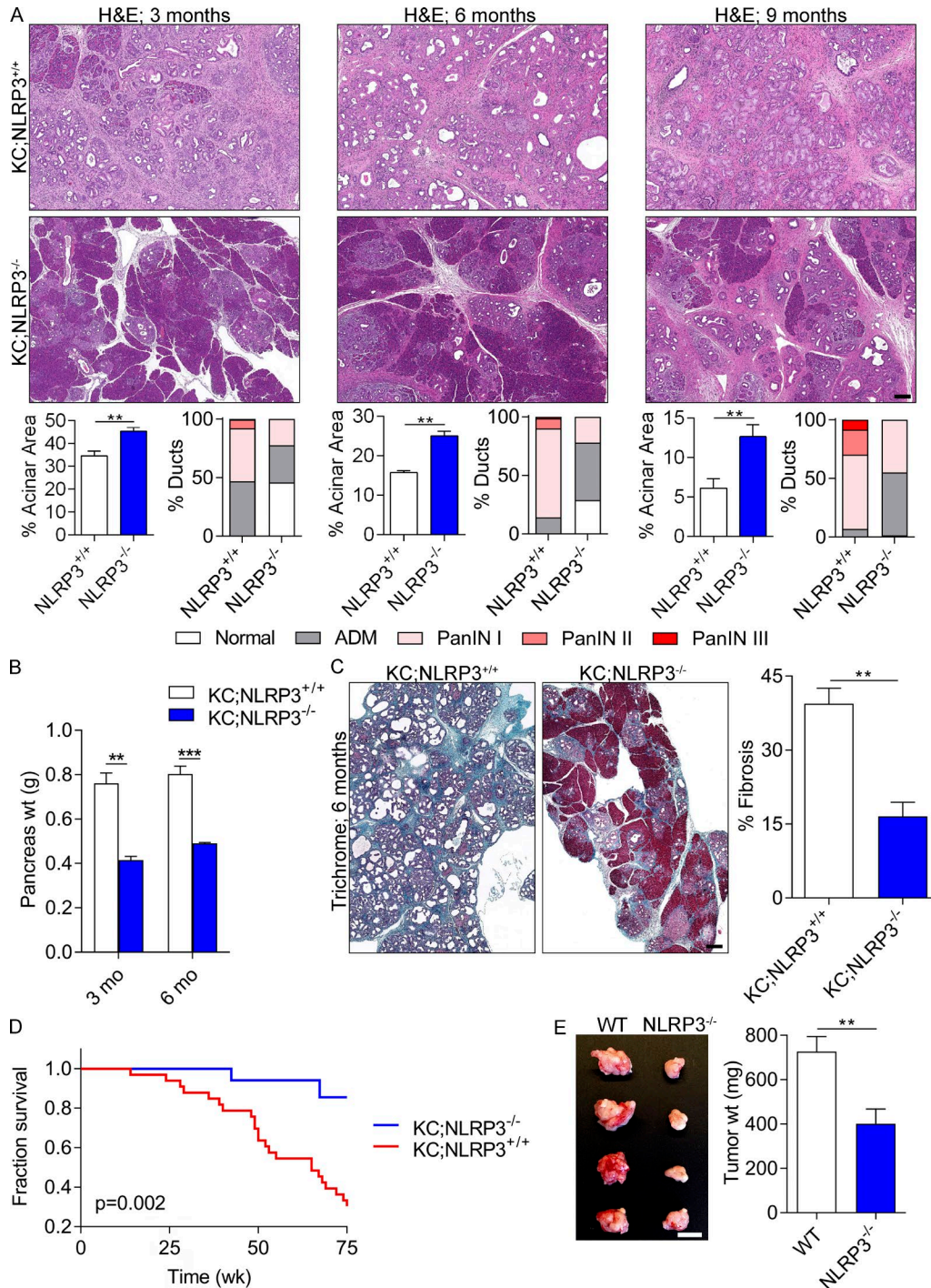
Figure 2. NLRP3 deletion or blockade is protective against PDA. (A) KC;NLRP3 +/+ and KC;NLRP3 -/- mice were sacrificed at 3, 6, or 9 mo of life (means of six to seven mice per time point). Representative H&E-stained sections are shown. The percentage of pancreatic area occupied by intact acinar structures and the fractions of ductal structures exhibiting normal morphology, acinoductal metaplasia (ADM), or graded pancreatic intraepithelial neoplasia (PanIN) I–III lesions were calculated. Bar, 200 \mu m. (B) Weights of pancreata were compared in 3- and 6-mo-old KC;NLRP3 +/+ and KC;NLRP3 -/- mice. (C) Pancreata of 6-mo-old KC;NLRP3 +/+ and KC;NLRP3 -/- mice were stained with trichrome, and the percentage of fibrotic pancreas' area was calculated. Bar, 200 \mu m. Unpaired Student's t test was used for statistical analyses. (D) Kaplan-Meier survival analysis was performed for KC;NLRP3 +/+ ( n = 29) and KC;NLRP3 -/- ( n = 24) mice. P = 0.002 based on the Wilcoxon test. (E) WT and NLRP3 -/- mice were challenged with orthotopically implanted KPC-derived tumor cells. Mice were sacrificed at 21 d, and pancreatic tumors were photographed and weighed. n = 8/group. Bar, 1 cm. Orthotopic tumor experiments were repeated more than five times with similar results. Unpaired Student's t test was used for statistical analyses. Mice were bred in house, and littermate controls were used. **, P < 0.01; ***, P < 0.001. Data are presented as mean \pm standard error.
