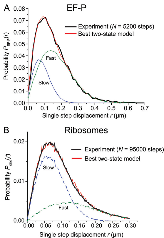
FIG 4 (A) Black, experimental probability distribution of single-step displacements taken by EF-P–mEos2 molecules in 2 ms. Red, the best fit to a static two-state model (without transitions) with D_{slow} constrained. Model parameters: D_{slow} = 0.2 \mu\text{m}^2/\text{s} ( \sigma_{slow} = 50 \text{ nm} ), f_{slow} = 0.30 , D_{fast} = 4.3 \mu\text{m}^2/\text{s} ( \sigma_{fast} = 75 \text{ nm} ), f_{fast} = 0.7 , with a \chi_r^2 = 1.0 . The individual slow and fast components are shown in dashed lines as labeled. (B) Black, experimental probability distribution of single-step displacements taken by ribosomes (30S labeled with mEos2) in 2 ms. Red, the best unconstrained fit to a static two-state model (without transitions). Model parameters: D_{slow} = 0.20 \mu\text{m}^2/\text{s} ( \sigma_{slow} = 40 \text{ nm} ), f_{slow} = 0.65 , D_{fast} = 0.8 \mu\text{m}^2/\text{s} ( \sigma_{fast} = 75 \text{ nm} ), f_{fast} = 0.35 , with \chi_r^2 = 2.3 . The slow and fast components are shown as dashed lines as labeled.
