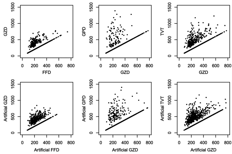
Figure 1. Scatter plots showing the relationships among measures for the Angele et al. data: GZD as a function of FFD (left), GPD as a function of GZD (middle), TVT as a function of GZD (right). The first row shows the real measures, the second the artificial measures. A subset of 1600 randomly selected data points (~50%) were used in this plot to improve readability.
