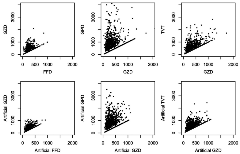
Figure 2. Scatter plots showing the relationships among measures for the Metzner et al. data: GZD as a function of FFD (left), GPD as a function of GZD (middle), TVT as a function of GZD (right). The first row shows the real measures, the second the artificial measures. A subset of 1600 randomly selected data points (~10%) were used in this plot to improve readability.
