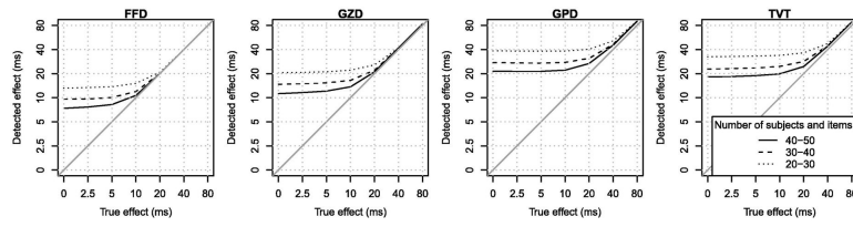
Figure 9. Size of detected effects as a function of true effect size for each eye-tracking measure and for different numbers of subjects and items. The grey line shows the result that we would expect from a (hypothetical) statistical test that is immune to Type M errors.
