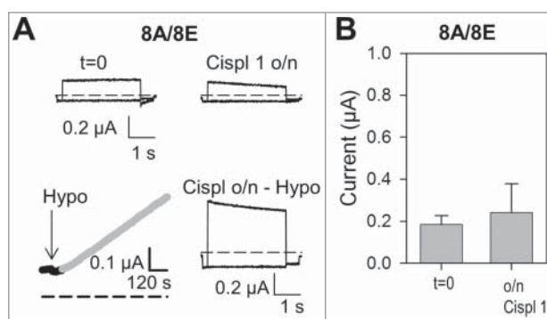
Figure 4. Cisplatin incubation does not alter currents of oocytes expressing WT 8A/8E. (A) Top: typical current traces measured in isotonic conditions of an 8A/8E expressing oocyte before and after overnight cisplatin incubation in the “maintaining” solution. Bottom: stimulation of the same oocyte after o/n incubation with hypotonic solution activates normal sized anion currents (left: current measured at 60 mV during hypotonic stimulation, right: voltage-clamp traces after hypotonic activation). (B) Mean values of 8A/8E currents in isotonic conditions before and after o/n cisplatin incubation ( n = 7 ; P > 0.05 ). Error bars indicate SD.
