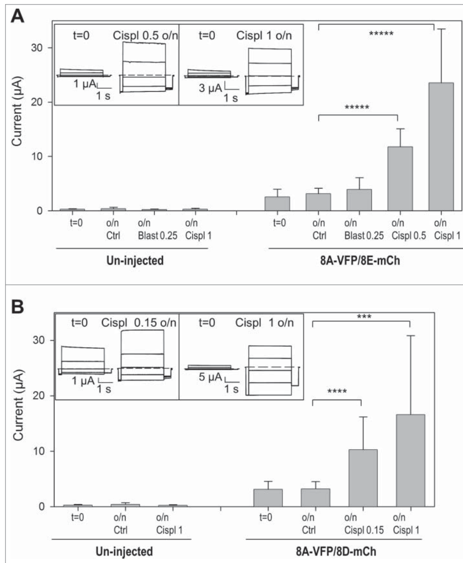
Figure 2. Cisplatin incubation strongly increases currents of oocytes expressing 8A-VFP/8E-mCh or 8A-VFP/8D-mCh. (A) Mean currents from un-injected or from 8A-VFP/8E-mCh injected oocytes measured before ( t = 0 ; un-injected n = 29 ; 8A-VFP/8E-mCh n = 60 ) and after overnight incubation in “Maintaining” solution (Ctrl; un-injected n = 11 ; 8A-VFP/8E-mCh n = 29 ), 0.25 mM blasticidin (Blast 0.25; un-injected n = 4 ; 8A-VFP/8E-mCh n = 9 ), 0.5 mM cisplatin (Cispl 0.5; 8A-VFP/8E-mCh n = 7 ) or 1 mM cisplatin (Cispl 1; un-injected n = 14 ; 8A-VFP/8E-mCh n = 15 ; **** P < 10^{-9} ). The insets show 8A-VFP/8E-mCh traces from one oocyte before and after overnight incubation in 0.5 mM (left) or 1 mM cisplatin (right). (B) Bars represent currents of un-injected or 8A-VFP/8D-mCh injected oocytes recorded before ( t = 0 ; un-injected n = 19 ; 8A-VFP/8D-mCh n = 39 ) and after overnight incubation in “Maintaining” solution (Ctrl; un-injected n = 8 ; 8A-VFP/8D-mCh n = 21 ), 0.15 mM cisplatin (Cispl 0.15; 8A-VFP/8D-mCh n = 6 ) or 1 mM cisplatin (Cispl 1; un-injected n = 11 ; 8A-VFP/8D-mCh n = 12 ; *** P < 0.001 ; **** P < 0.0001 ). The insets show typical 8A-VFP/8D-mCh traces from one oocyte before and after overnight incubation in 0.15 mM (left) or 1 mM cisplatin (right). Error bars indicate SD.
