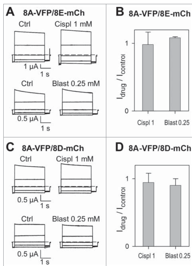
Figure 1. Acute application of cisplatin and blasticidin does not affect currents mediated by 8A-VFP/8E-mCh or 8A-VFP/8D-mCh. (A) Typical current traces of 8A-VFP/8E-mCh expressing oocytes evoked by the “IV-pulse protocol” (see Materials and Methods) in control conditions and after perfusion of 1 mM cisplatin (top) or 0.25 mM blasticidin (bottom). (B) 8A-VFP/8E-mCh currents measured at 60 mV in presence of 1mM cisplatin or 0.25 mM blasticidin were normalized to the value measured before drug application ( n = 5 for cisplatin; n = 3 for blasticidin). (C-D) Acute effect of cisplatin and blasticidin on 8A-VFP/8D-mCh. (C) Voltage clamp traces of oocytes expressing 8A-VFP/8D-mCh before and after perfusion of 1 mM cisplatin (top) or 0.25 mM blasticidin (bottom). (D) 8A-VFP/8D-mCh currents recorded at 60 mV were normalized to the value measured before drug application ( n = 3 ). Error bars indicate SD.
