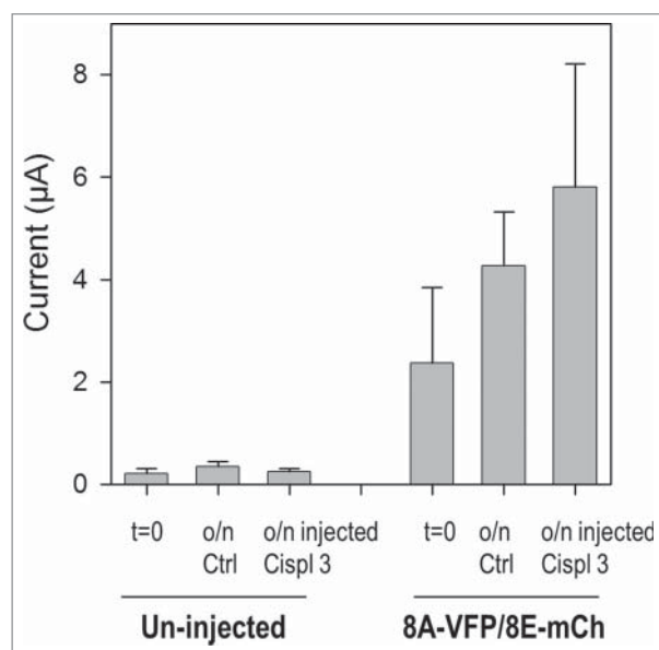
Figure 3. Cisplatin injection does not modify 8A-VFP/8E-mCh currents. Bars represent mean currents of un-injected or 8A-VFP/8E-mCh injected oocytes measured before ( t = 0 ; un-injected n = 11 ; 8A-VFP/8E-mCh n = 15 ) and after overnight incubation in “Maintaining” solution. After recording currents in control conditions, some oocytes were just incubated (o/n Ctrl; un-injected n = 4 ; 8A-VFP/8E-mCh n = 8 ), others were injected with 50 nl of a 3 mM cisplatin solution and then incubated overnight (o/n inj Cispl 3; un-injected n = 7 ; 8A-VFP/8E-mCh n = 7 ; P > 0.05 ). Error bars indicate SD.
