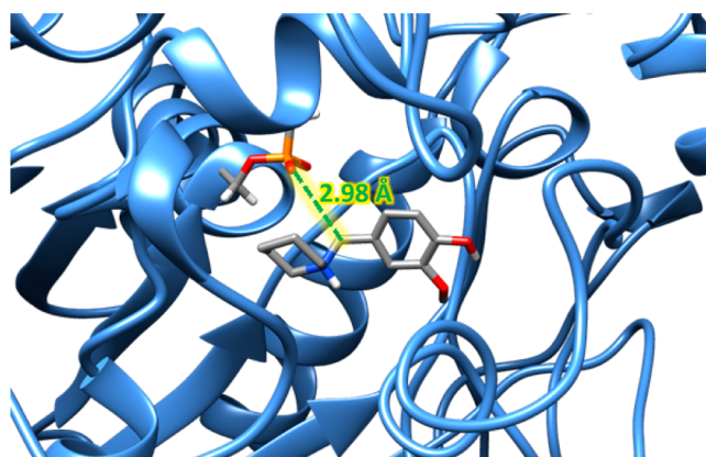
Figure 2. Docked pose of 3-HCl in the aged AChE active site, displaying the putative reactive orientation of the benzylic carbon being less than 5 Å from aged serine residue.
