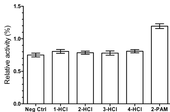
Figure 3. Result of AChE realkylation test. The relative activity of 2-PAM control was 1.2%, implying the near completeness of aging. Aged AChE samples treated with tested QMPs were not obviously more active than the negative control (Neg Ctrl).
