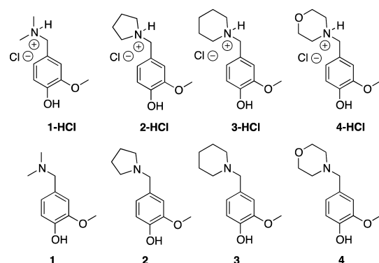
Figure 1. Target quinone methide precursors.
