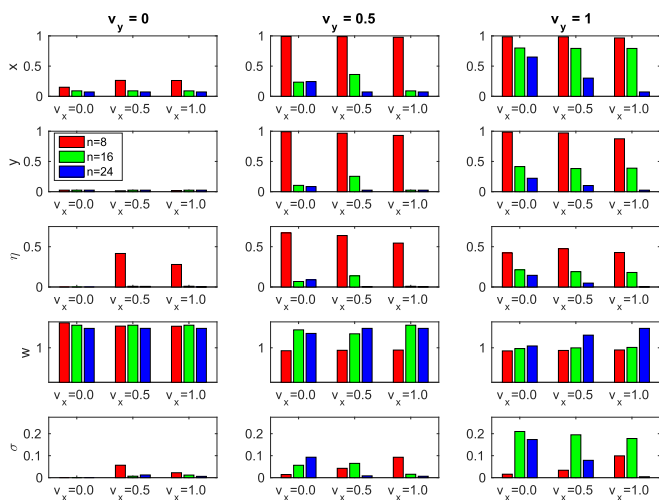
Fig. 4. Summary graphs for us-vs.-them games: efforts x , punishment y , internalization \eta , fitness w , and SD \sigma in internalization trait \eta for different normative values of production v_x and punishment v_y , and group size n . Other parameters: \delta = 0.5 , b = 1 , K = 3 . Shown are averages based on 10 runs for each parameter combination.
