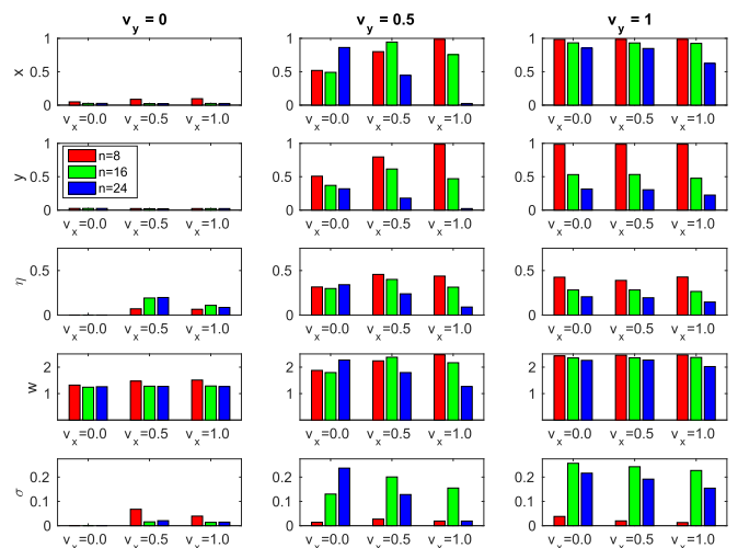
Fig. 3. Summary graphs for us-vs.-nature games: efforts x , punishment \eta , fitness w , and SD \sigma in internalization trait \eta for different normative values of production v_x and punishment v_y , and group size n . Other parameters: X_0 = n/2 , \delta = 0.5 , b = 4 , K = 3 . Shown are averages based on 10 runs for each parameter combination.
