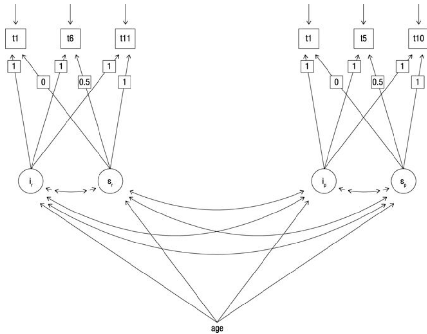
Figure 2. Bivariate latent growth curve model of risk-taking propensity and the Big Five personality traits. The observed variables t1 , t6 , and t11 (and t1 , t5 , and t10 ) represent the repeated measurements of risk-taking propensity (left) and the Big Five personality traits (right). Whereas risk-taking propensity was measured by one item, three items for each trait measured the Big Five. Therefore, for personality, the measurements at t1 , t5 , and t10 were again latent factors composed of these three items. Two-headed arrows represent correlations, single-headed arrows regression coefficients. The latent intercept ( i ) is fixed to 1 on t1 , t5 , and t10 and refers to the estimated mean frequency of risk-taking propensity at t1 . The latent slope ( s ) is fixed to 0.00 on t1 , to 0.50 on t5/t6 , and to 1 on t10 and refers to the estimated mean difference between two neighboring measurement points. Age was included as predictors of i and s .
