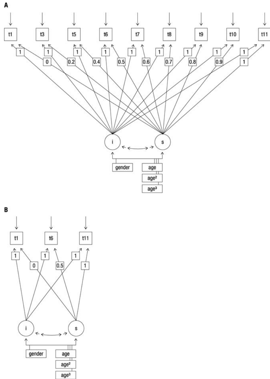
Figure 1. Model representation of the latent change model used to analyze effects of age and sex on the mean level (intercept) and mean-level change (slope) of self-reported domain-general (A) and domain-specific (B) risk propensity (2004–2014). A. At each measurement point (t1 to t11) one item was assessed. The latent intercept ( i ) is fixed to 1 on t1, t3, t5, t6, t7, t8, t9, t10, and t11 and refers to the estimated mean frequency of risk-taking propensity at t1. The latent slope ( s ) is fixed to 0.00 on t1, to 0.20 on t3, to 0.40 on t5, to 0.50 on t6, to 0.60 on t7, to 0.70 on t8, 0.80 on t9, to 0.90 on t10, and to 1 on t11 and refers to the estimated mean difference between two neighboring measurement points. Two-headed arrows represent correlations; single-headed arrows, regression coefficients. Gender, age, age 2 , and age 3 were included as predictors of ( i ) and ( s ). B. At each measurement point (t1, t5, t10) one item was assessed. The latent intercept ( i ) is fixed to 1 on t1, t5, and t10 and refers to the estimated
