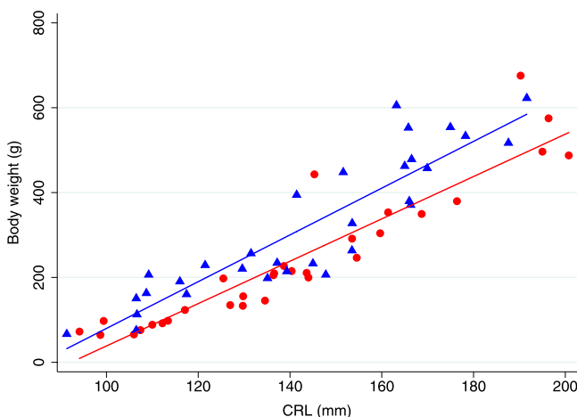
Figure 1. Body weight (g) as a function of CRL (mm) in Japanese monkey fetuses pre- and post-NPP disaster (n = 62). The figure shows regressions between body weight and CRL in pre- and post-disaster groups. Blue triangles were pre-disaster monkey fetuses with the blue line representing the fitted values (n = 31); R^2 = 0.86 . Red circles were post-disaster monkey fetuses with the red line representing the fitted values (n = 31); R^2 = 0.82 .
