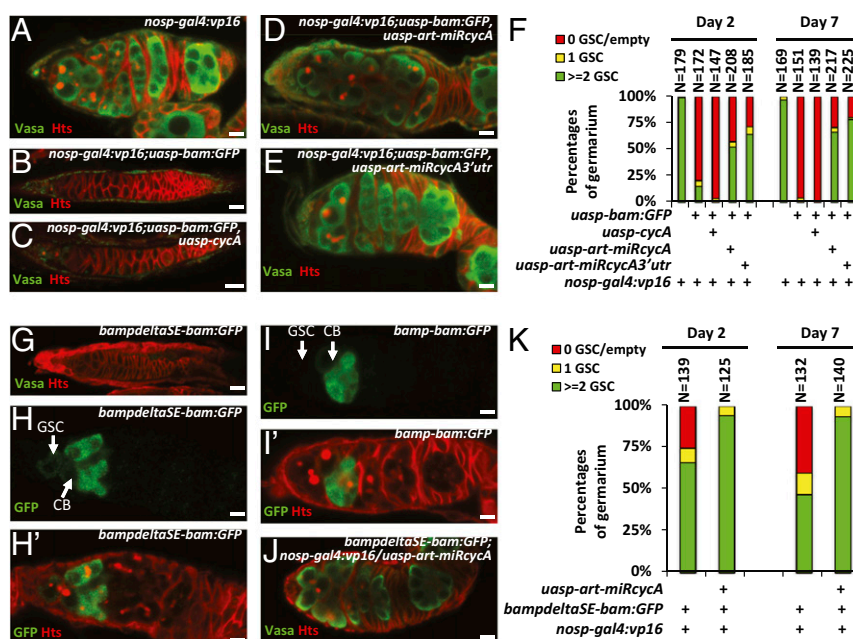
Fig. 3. CycA is a downstream target of Bam. (A–E) Ovaries from P{nosp-gal4:vp16} (A, wild-type control), P{nosp-gal4:vp16};P{uasp-bam:GFP}/P{uasp-cycA} (C), P{nosp-gal4:vp16};P{uasp-bam:GFP}/P{uasp-art-miRcycA} (D), and P{nosp-gal4:vp16};P{uasp-bam:GFP}/P{uasp-art-miRcycA3'utr} (E) were stained with anti-Vasa (green) and anti-Hts (red) antibodies. Vasa was used to visualize germ cells. Hts was used to outline the germarium and morphology of fusomes. (F) Quantification of the germarium phenotypes of ovaries in A–E. (G and J) Ovaries of P{bampdeltaSE-bam:GFP} (G) and P{nosp-gal4:vp16};P{bampdeltaSE-bam:GFP}/P{uasp-art-miRcycA} (J) were stained with anti-Vasa (green) and anti-Hts (red) antibodies. (H–I) Ovaries of P{bampdeltaSE-bam:GFP} (H and H') and P{bamp-bam:GFP} (I and I') were stained with anti-GFP (green) and anti-Hts (red) antibodies. (Scale bars: 10 \mu m.) (K) Statistical quantification of the germarium phenotypes of ovaries in G and J.
